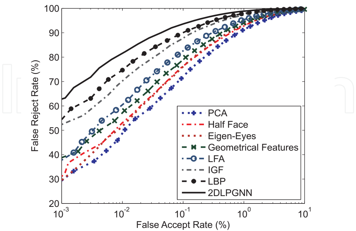
Fig. 12. ROC to evaluate the performance of face recognition algorithms on the face disguise database
