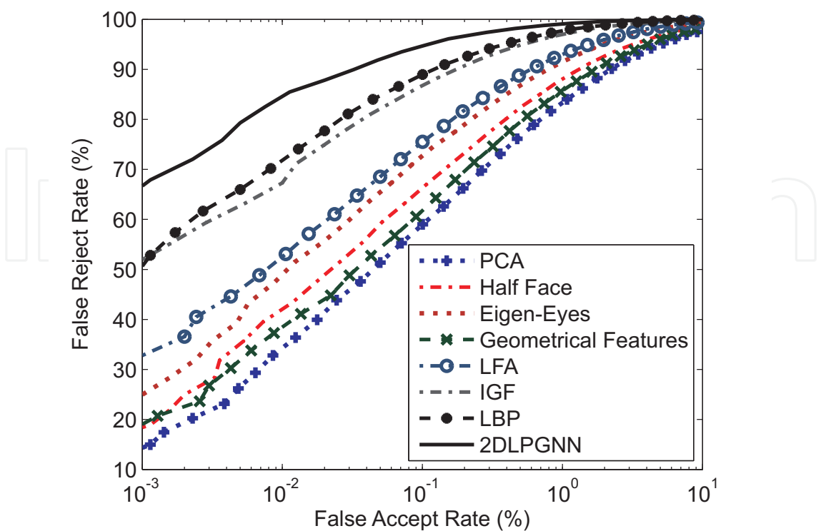
Fig. 11. ROC to evaluate the performance of face recognition algorithms on the heterogeneous face database
