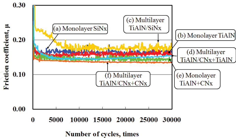
Figure 17. Average friction coefficients for monolayer and multilayer films under dry conditions and water and PAO lubrication.
