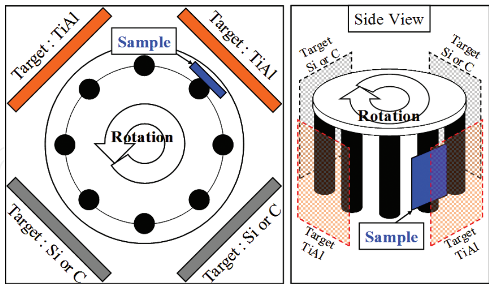
Figure 1. Schematic of DC sputtering equipment.
