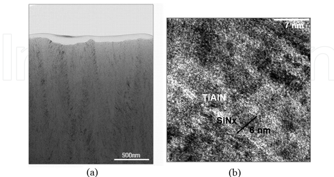
Figure 5. Cross-sectional TEM images of TiAlN/SiN coating, observed at scale of (a) 500 nm and (b) 7 nm.
