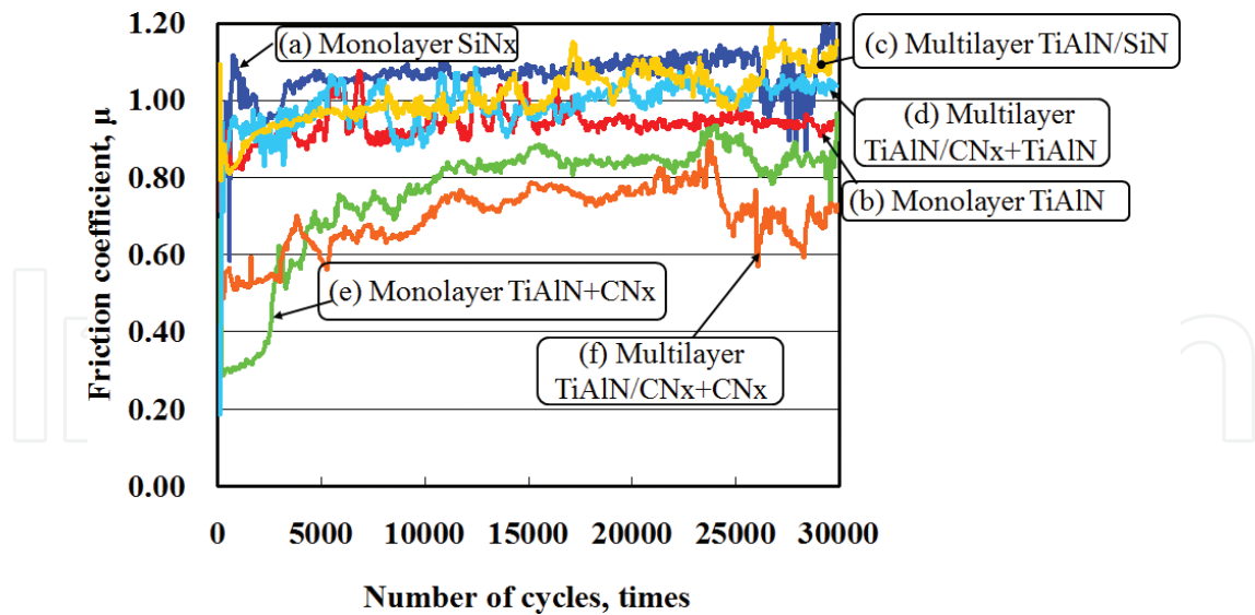
Figure 9. Friction coefficient vs. number of sliding cycles for the SRV friction test under dry conditions for: (a) SiNx, (b) TiAlN, (c) TiAlN/SiN, (d) TiAlN/CNx + TiAlN, (e) TiAlN + CNx, and (f) TiAlN/CNx + CNx coatings.
