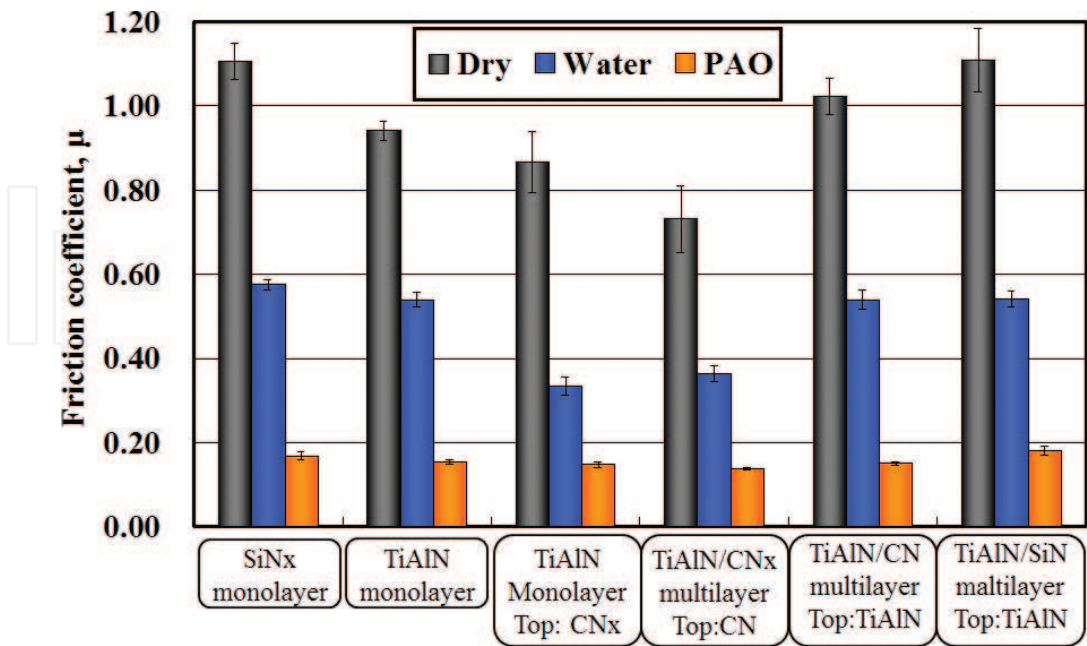
Figure 19. Average friction coefficients for monolayer and multilayer films under dry conditions and water and PAO lubrication.
