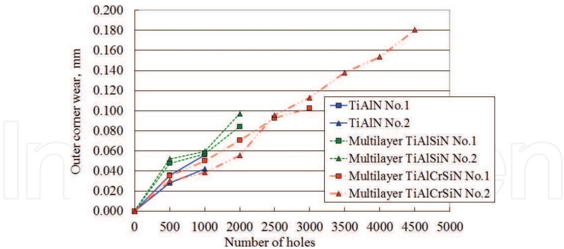
Figure 22. Outer corner wear of 6-mm diameter WC-co drills as a function of the number of holes drilled. Cutting speed: 100 m/min (5304 rpm), feed rate: 0.18 mm/rev. Workpiece: Carbon steel (S50C). Cutting fluid: Water soluble agent. Hole depth 30 mm (5×diameter).
