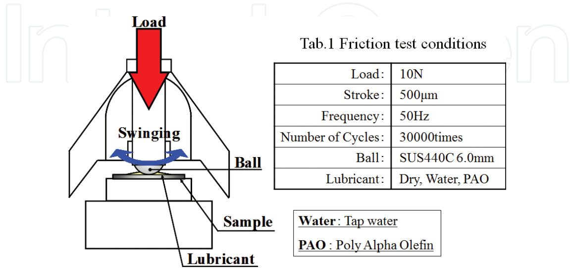
Figure 3. Swing type friction tester (SRV).
