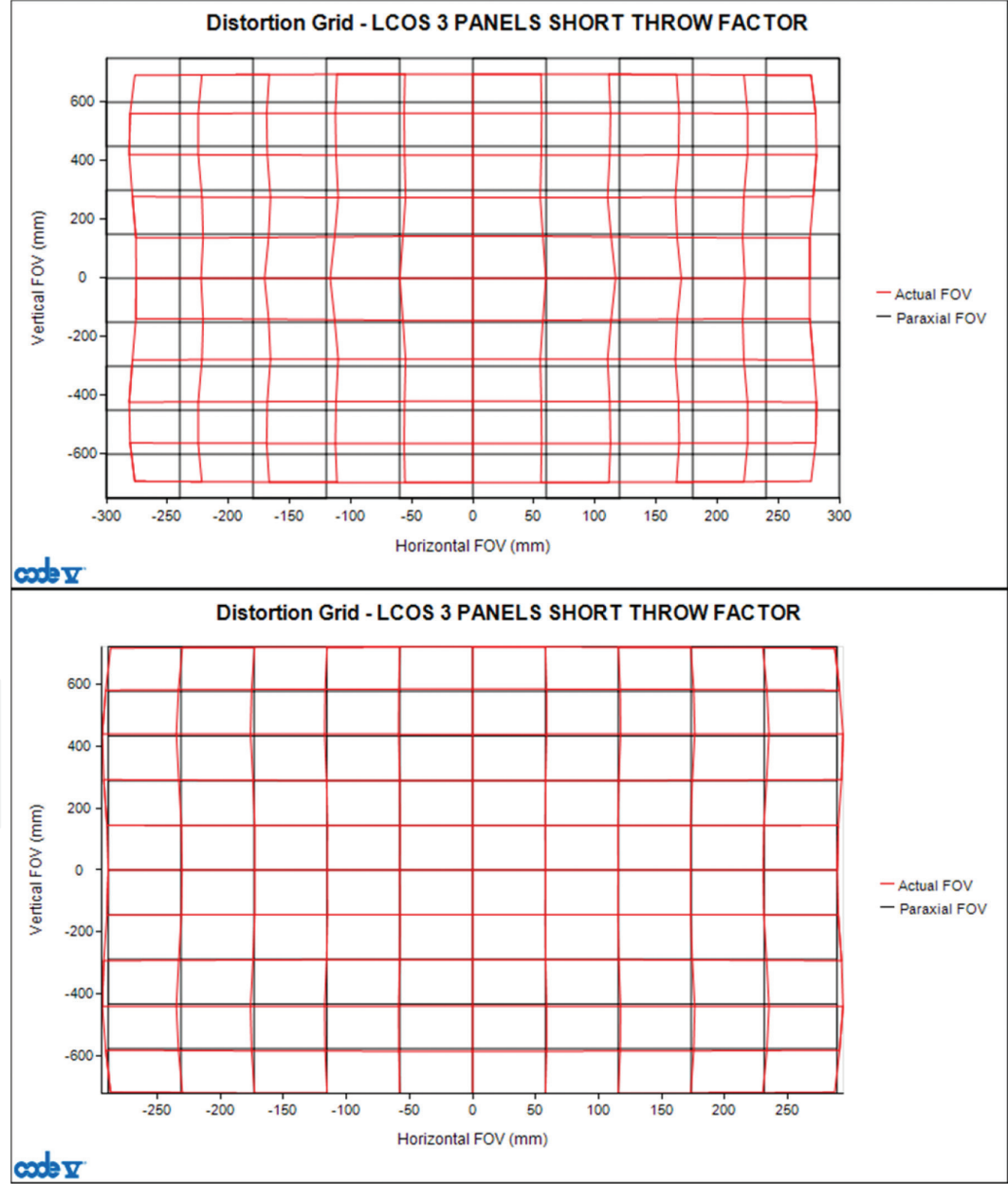
Figure 16. The distortion before and after tuning the optical parameter.
