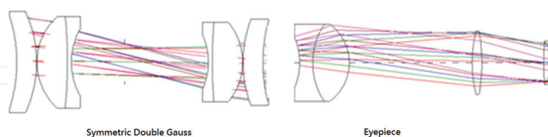
Figure 8. Symmetric double gauss and wide eye-piece types.
