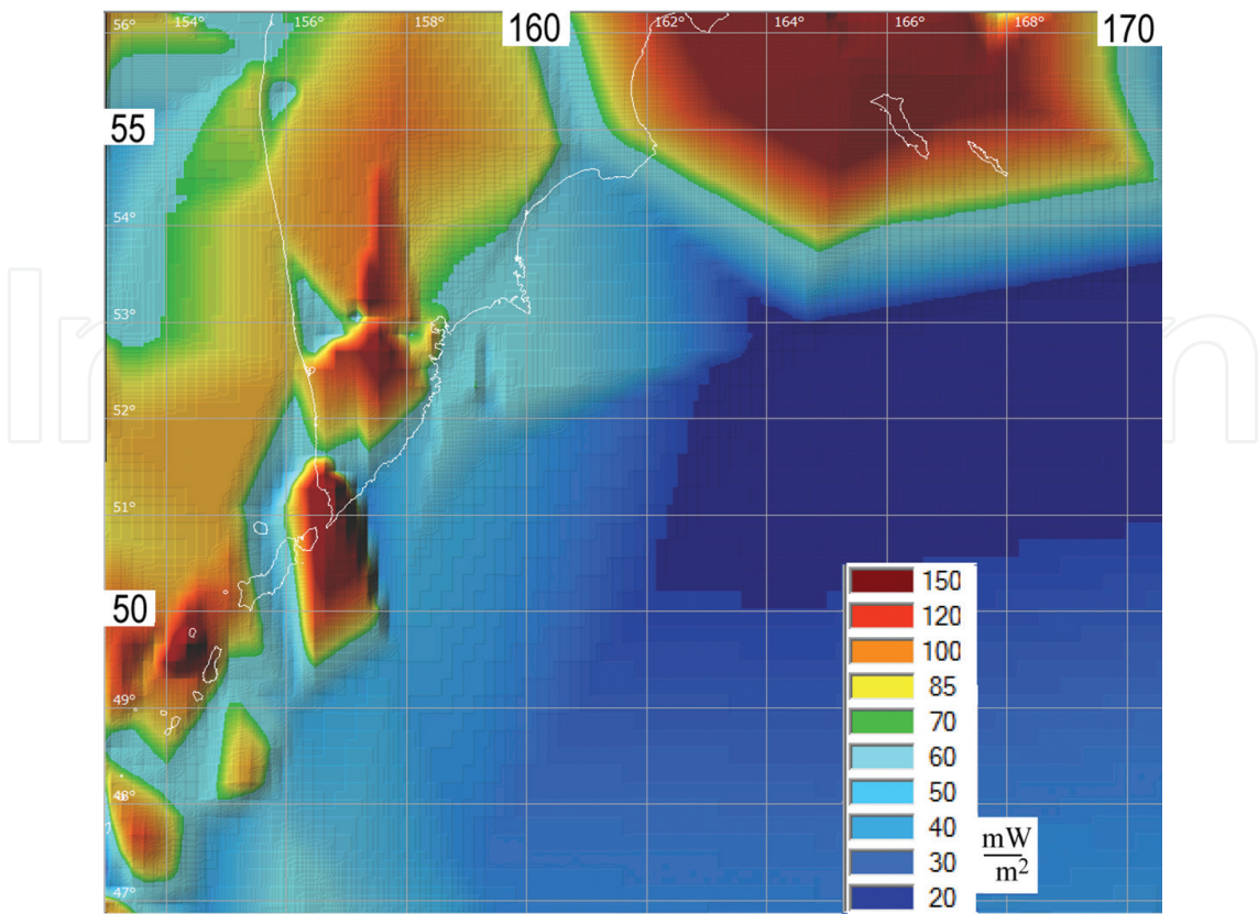
Figure 5. The regional thermal field in the morphostructures of the Kamchatka region and associated volcanic arcs.
