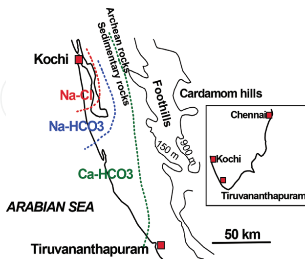
Figure 1. Water types in the Kerala Tertiary coastal aquifer resulting from flushing by recharge before the Last Glacial Maximum. The Precambrian, under-lying the Tertiary strata, are faulted in the SE-NW direction, which also guides the recharge in the same direction.
