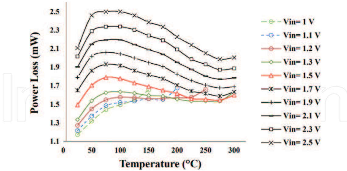
Figure 12. Power losses as a function of temperature.
