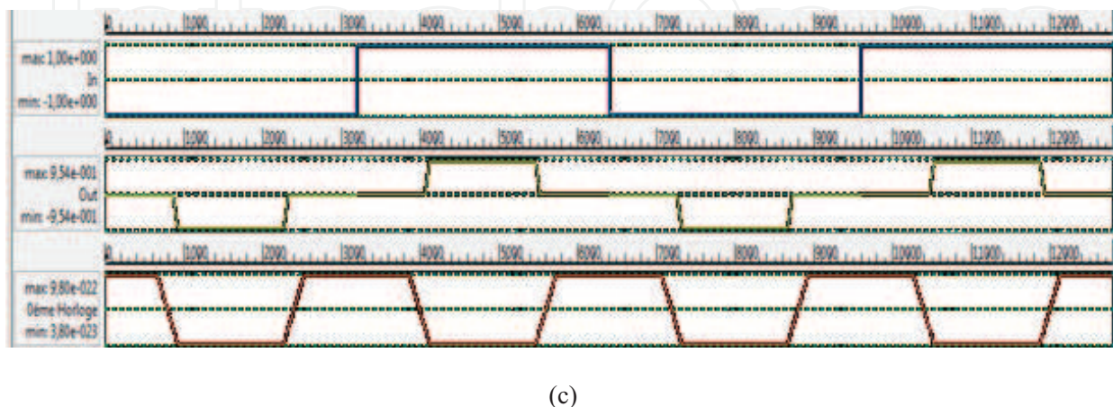
Figure 5. Binary wire, (a) representation, (b) QCA layout, and (c) simulation results.
