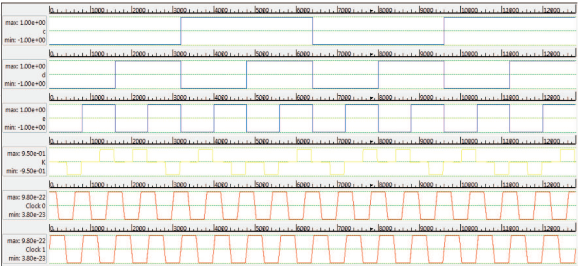
Figure 19. The simulation result of the novel architecture of 3-input “XOR” gate.
