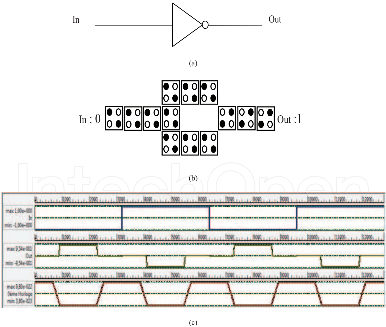
Figure 6. Inverter gate, (a) representation, (b) QCA layout, and (c) simulation results.
