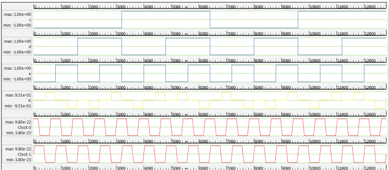
Figure 14. The simulation result of the novel architecture of 3-input logical “XNOR” gate.
