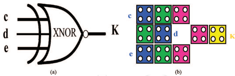
Figure 13. Schematic of 3-input “XNOR” gate. (a) Schematic of “XNOR” gate and (b) QCA layout of proposed “XNOR” gate.
