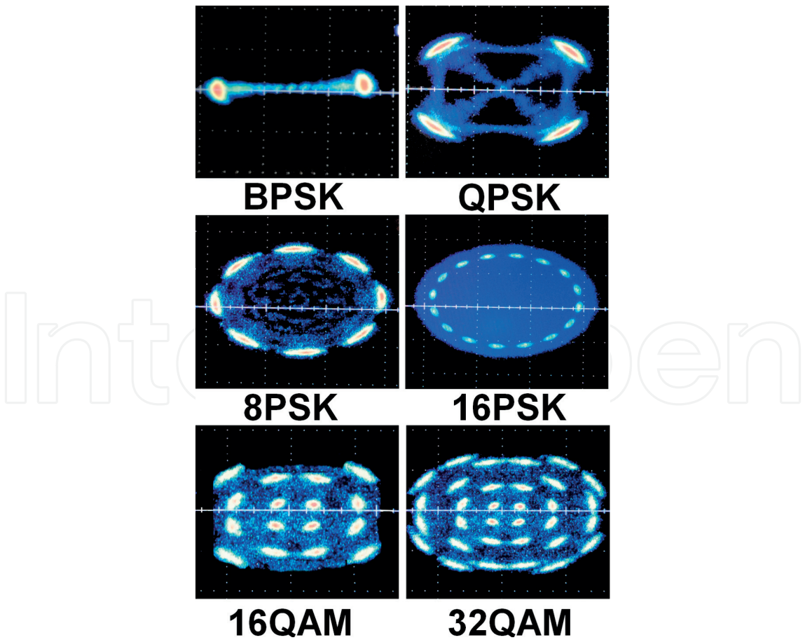
Figure 21. Experimental constellation results of the demodulated MPSK/MQAM signals.
