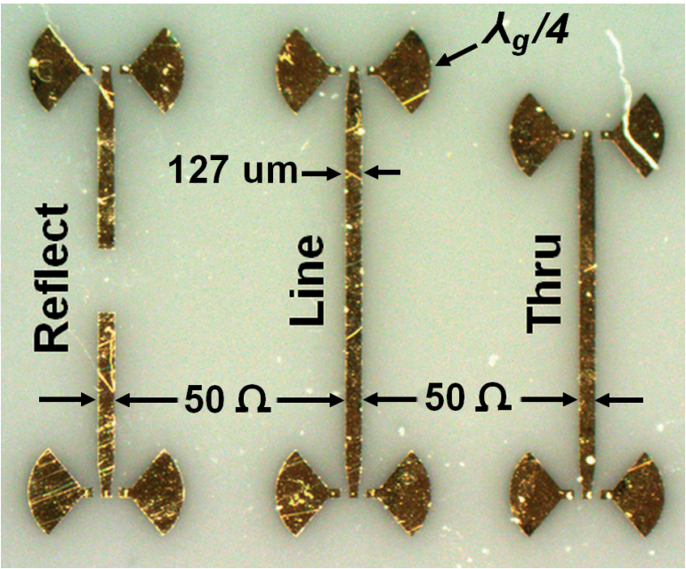
Figure 3. Microphotograph of TRL calibration kit.
