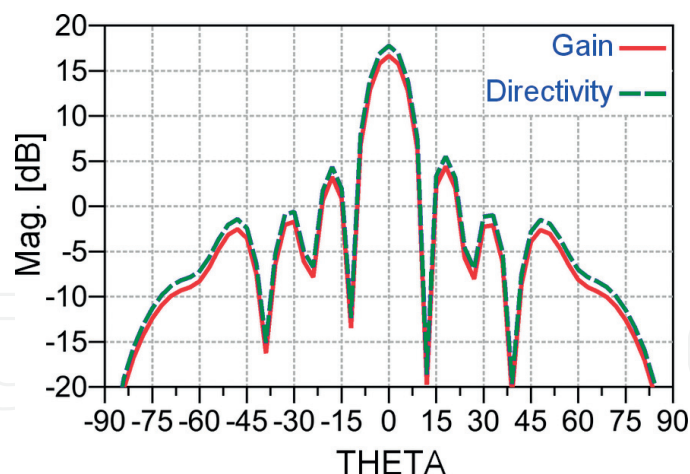
Figure 17. 2D simulated radiation pattern of the proposed 8 \times 2 microstrip antenna array at 60.5 GHz.
