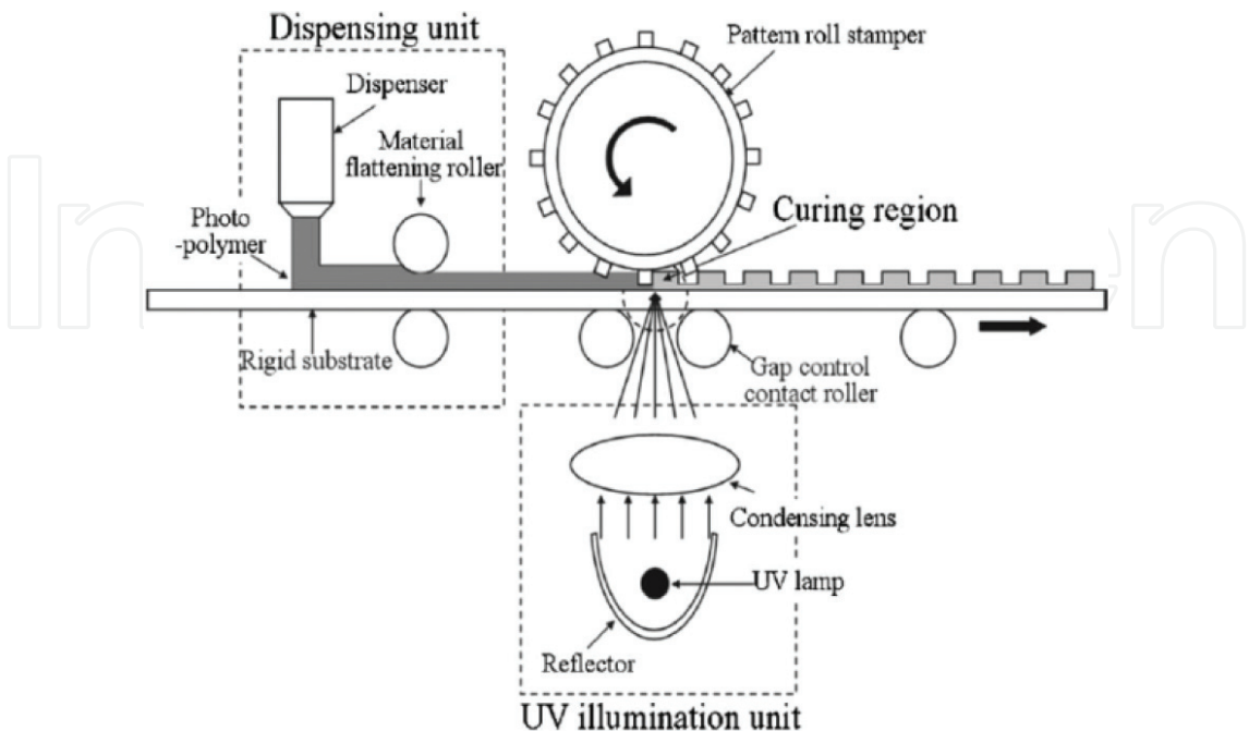
Figure 7. Schematic of R2P UV-NIL process for a rigid and transparent substrate developed by Ahn et al. [25].
