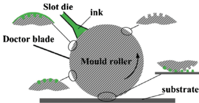
Figure 10. Schematic diagram of roller-reversal imprint process [28].
