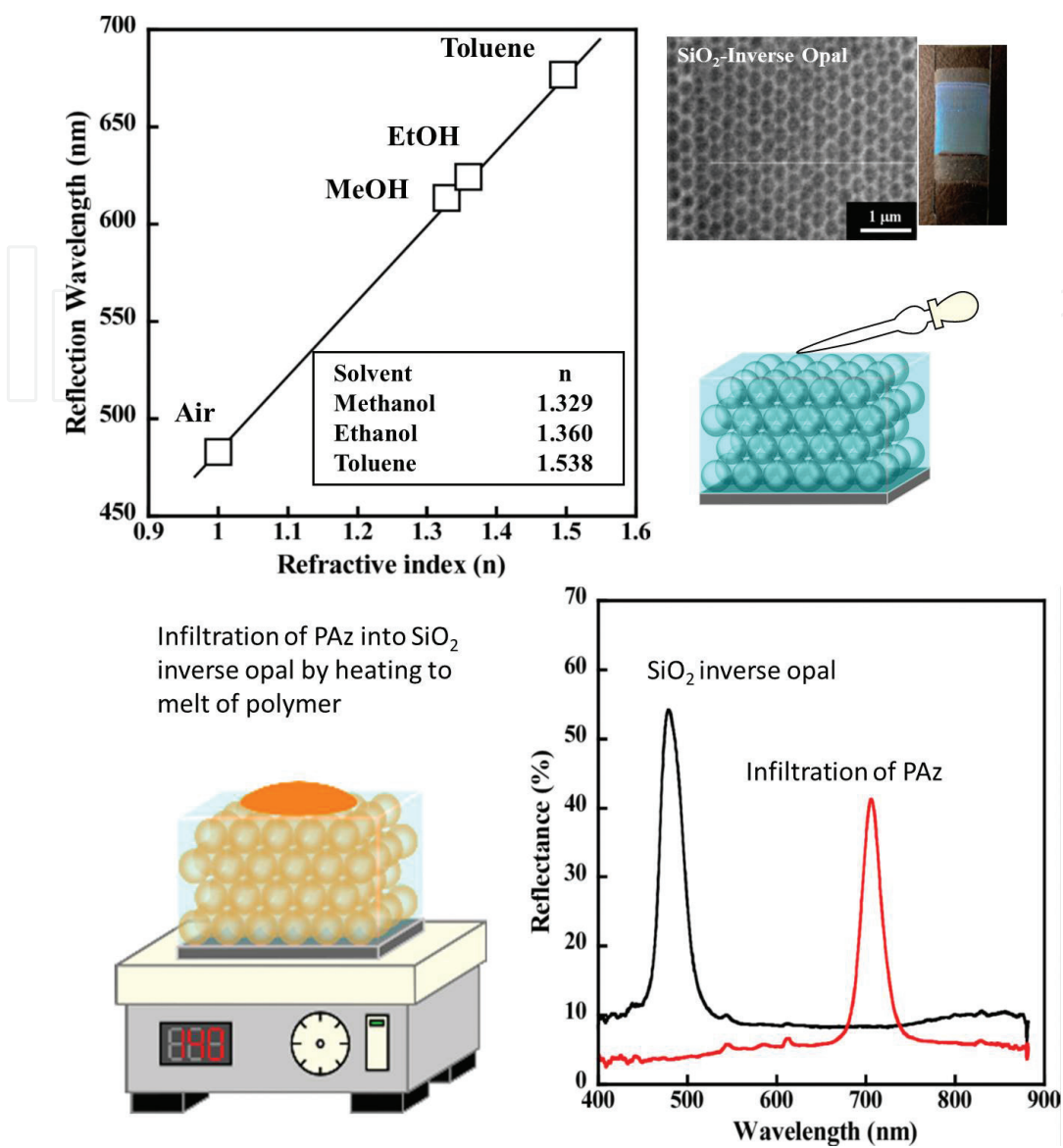
Figure 8. Plot of reflection wavelength change of SiO 2 inverse opal structure depending on solvents with various refractive indices (a) and reflection spectra before and after infiltration of PAz (b).
