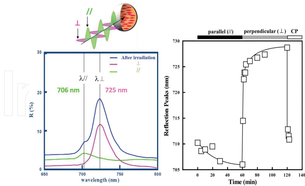
Figure 9. Reflection spectra of Paz-infiltrated \text{SiO}_2 film with parallel and perpendicular LPL irradiation of Ar + laser and plot of the wavelength of reflection peak [59].
