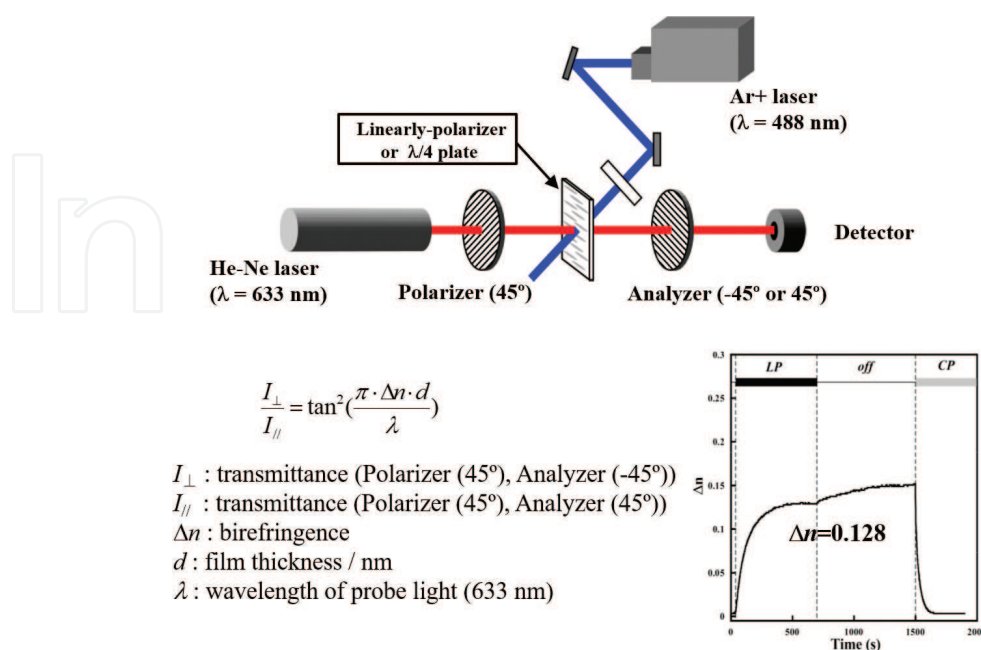
Figure 7. Schematic for birefringence measurement and the result of PAz.
