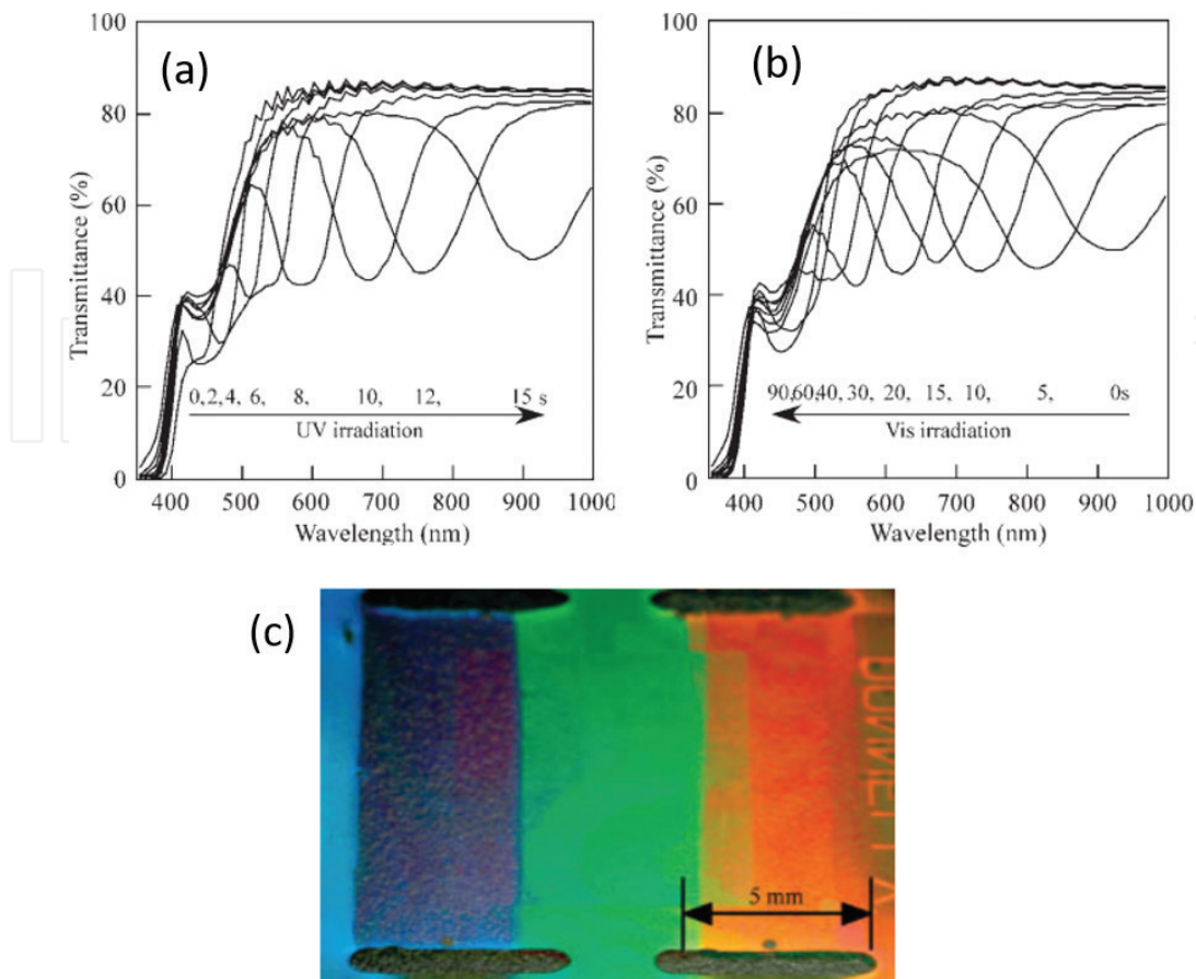
Figure 1. Changes in the selective reflection of the ChLC after UV irradiation (a) and visible light (b) irradiation at 25°C. And the photograph (c) of color change of the ChLC by varying UV irradiation time 0 s (left), 4 s (middle), and 10 s (right). [31] Copyright 2005, Wiley-VCH.
