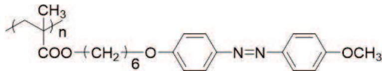
Figure 5. Schematic molecular structure of PAz.
