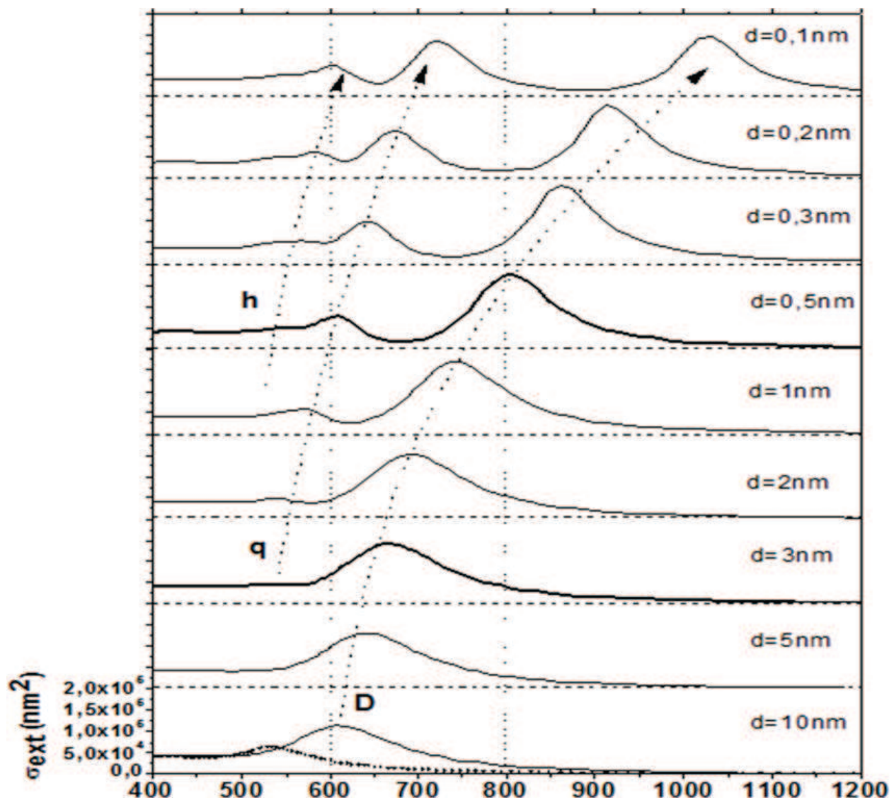
Figure 12. Extinction spectra (longitudinal excitation) of gold dimers ( R = 50 nm, n_m = 1.15 ) calculated by the generalized Mie theory as a function of the interparticle distance d . The dotted spectrum (for d = 10 nm) is obtained for transverse excitation. To guide the eye, dotted arrows indicate the redshift of the dipolar (D), quadrupolar (q) and hexapolar (h) resonance. The spectra for d = 0.5 nm and d = 3 nm are highlighted.
