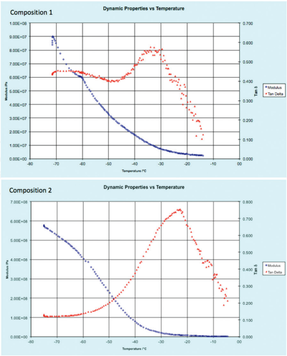
Figure 12. DMTA results of the Comp. 1 and Comp. 2.
