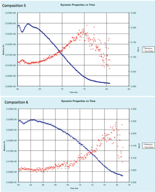
Figure 14. DMTA results of the Comp. 5 and Comp. 6.
