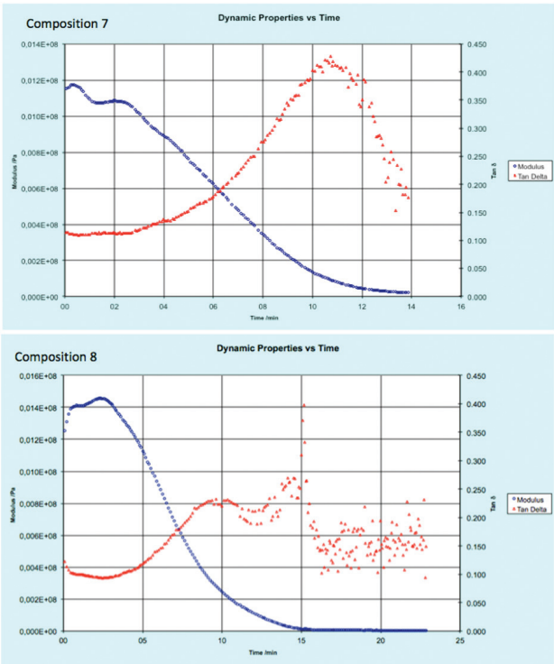
Figure 15. DMTA results of the Comp. 7 and Comp. 8.
