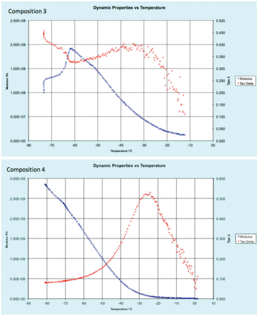
Figure 13. DMTA results of the Comp. 3 and Comp. 4.
