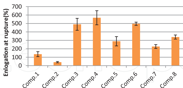
Figure 3. Results of elongation at rupture (%).
