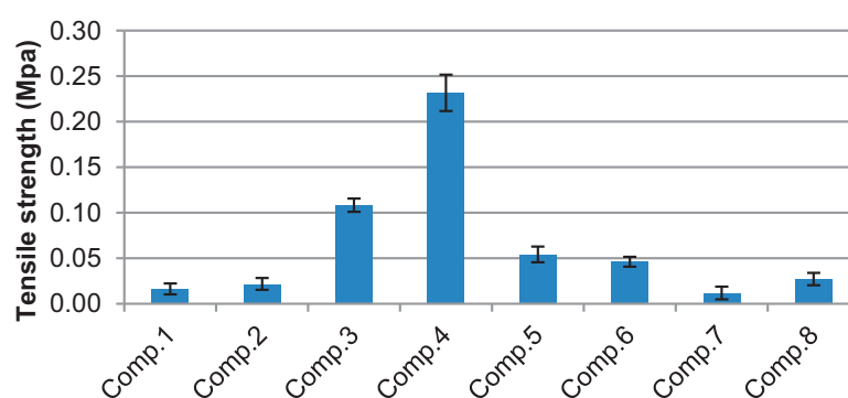
Figure 2. Results of the tensile strength.
