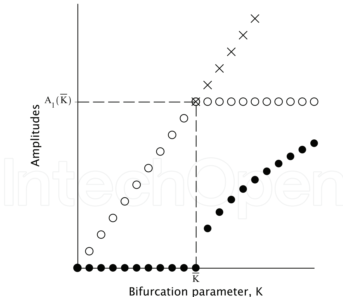
Figure 1. Bifurcation diagram—Amplitudes of radial and angular modes versus control parameter K . Solid circles refer to stable angular oscillations, circles mark stable radial oscillations. Crosses denote unstable radial mode. Change in the stability takes place near the bifurcation point \bar{K} (parameter \Lambda = 3/8\sqrt{2} has been scaled arbitrary for the best view).
