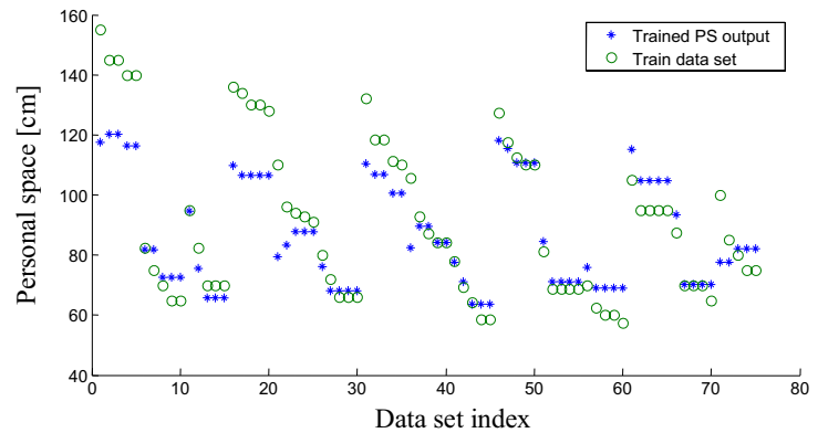
Figure 11. Trained ANFIS output with train data set values
