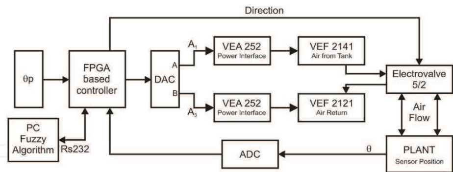
Fig. 6. Control block diagram for single-link flexible manipulator with pneumatic actuator. Figure 7 shows a block diagram of hardware description to be implemented into FPGA, such as DAC driver, ADC driver, 50 ms sample time generator, communication protocol controller (RS232 driver), a register to load the DAC input (Register) and the finite state machine to synchronize each module (FSM control).
