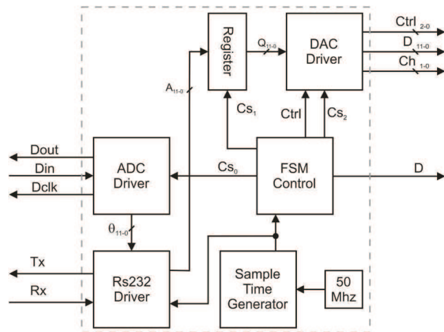
Fig. 7. Hardware description for FPGA block diagram. The FPGA is used to implement the digital interface to control the flexible manipulator robot prototype that is shown in figure 8. Figure 9 shows the hardware used to control the flexible manipulator development.
