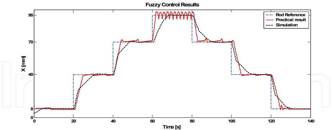
Fig. 10. Fuzzy control behavior of the flexible arm.
