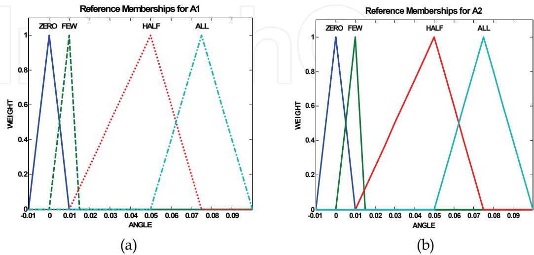
Fig. 5. Membership functions for the valve values. (a) Valve 1. (b) Valve 2.
