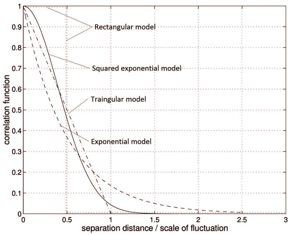
Figure 2. Four correlation functions for correlation models defined in Table 1.
