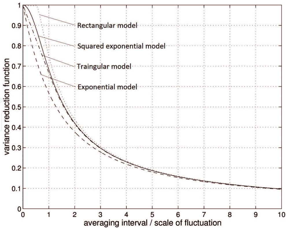
Figure 3. Four variance reduction functions for correlation models defined in Table 1.
