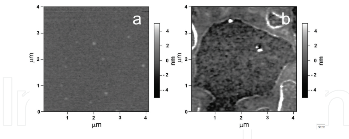
Figure 3. AFM images of HA plasma polymer films deposited with a power of 50 W: (a) as deposited or (b) after immersion in water for 24 h.
