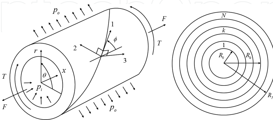
Figure 2. A laminated tube and the defined coordinate systems.
