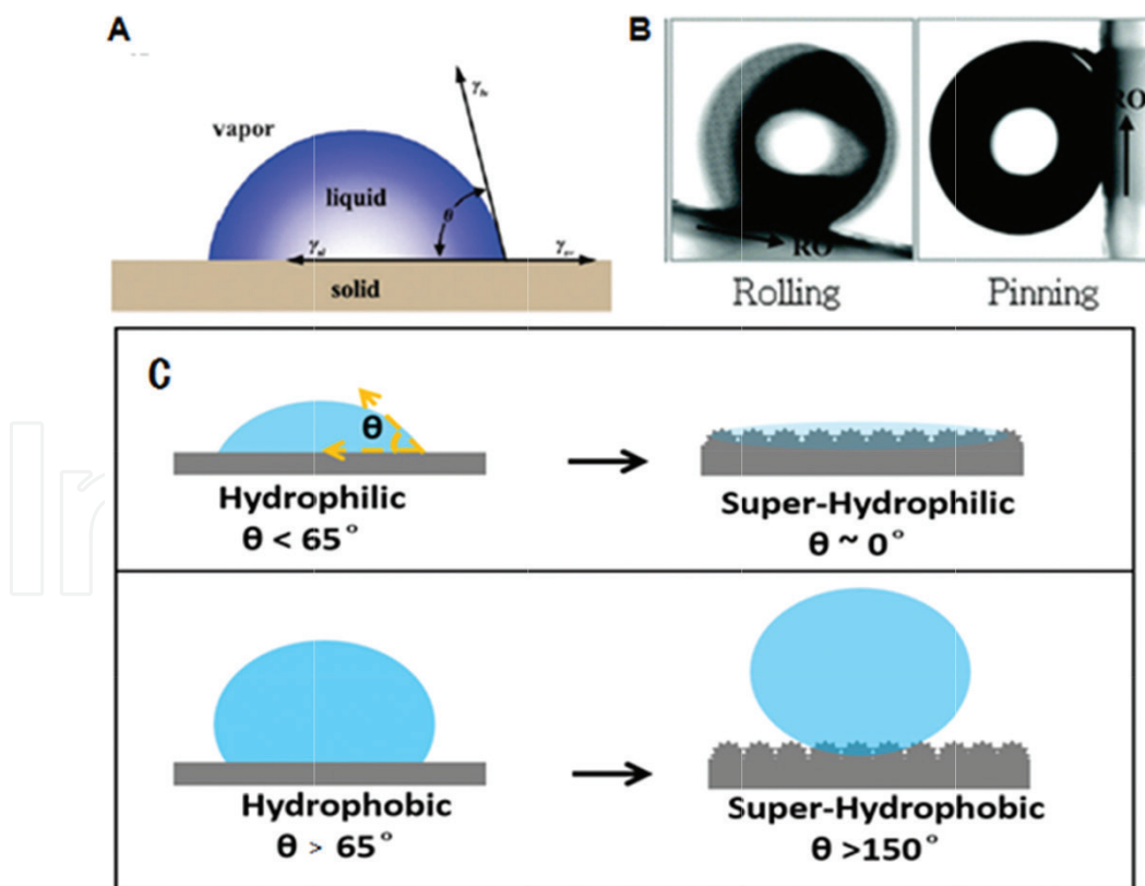
Figure 2. Wettability of interfaces. (A) Statistic contact angle, (B) sliding angle with different substrate adhesive, (C) schematic illustration of different wettability state [35].
