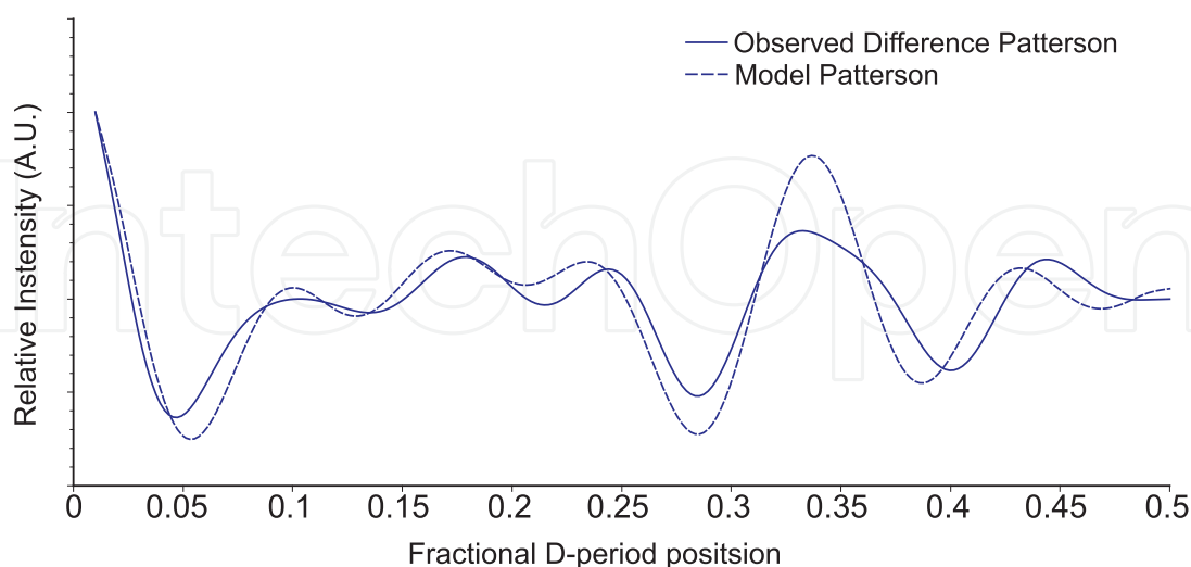
Figure 8. Model vs. observed difference Patterson maps. Difference Patterson map between glycated and non-glycated tendons with DPBA (solid blue line) along 1D period represented in fractional positions. The peak positions show the distances between electron dense regions seen in the difference Fourier map ( Figure 7 ). The similarity model Patterson (dashed blue line) confirms that the scaling of derivative amplitudes from the XRD patterns and the application of native phases is appropriate, thus validating the sequence and structure specific interpretations.
