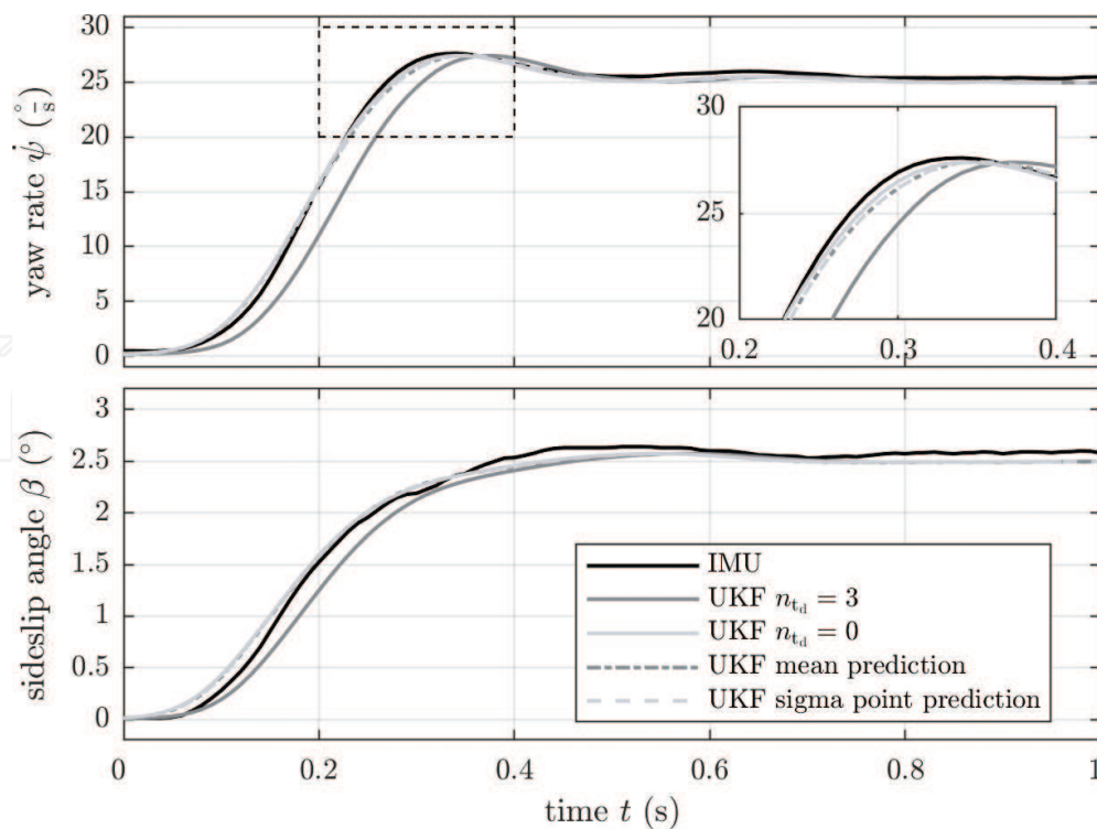
Figure 8. Dead-time-compensated vehicle state estimation during step steering maneuver.
