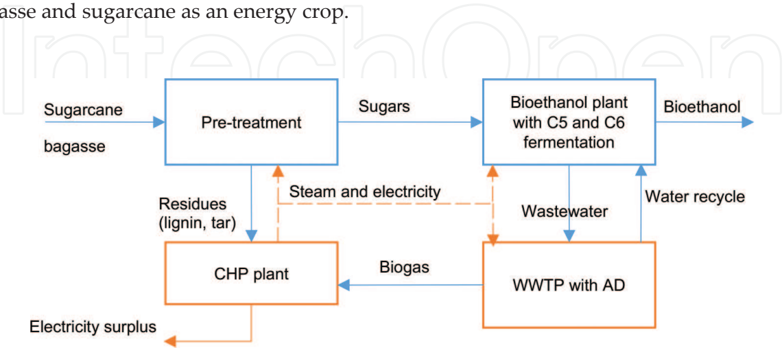
Figure 3. Integrated system for bioethanol production from sugarcane bagasse.
