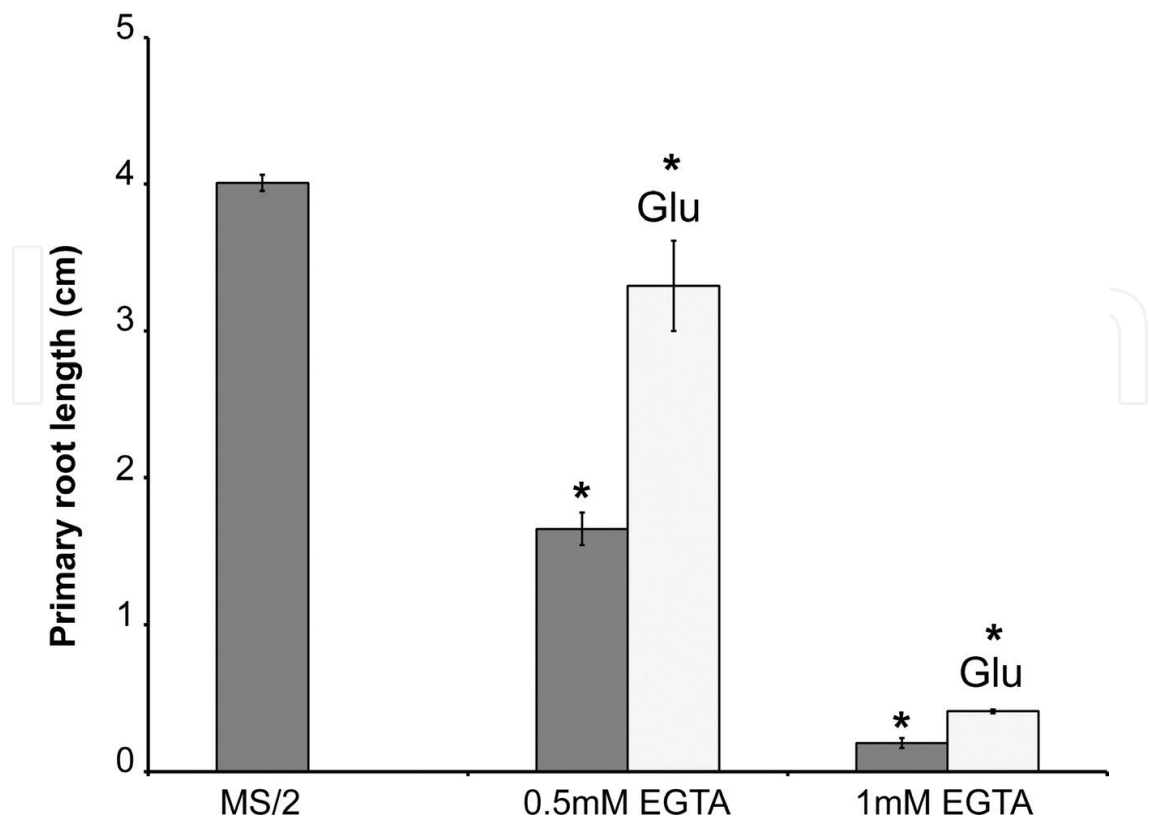
Figure 4. \text{Ca}^{2+} -dependent growth phenotypes of EGTA treated wild-type root seedlings. Putative ligand Glu can overcome reduced root growth by low amount of EGTA. Root phenotype of the 10-day-old wild-type seedlings under the different treatments. Supplement of 0.5 mM Glu successfully recovered the primary root growth which was reduced by 0.5 mM and 1 mM EGTA. The data presented are averages of three biological replicates. Asterisks represent statistical difference analyzed with a Student's t -test; P < 0.005 , n = 15 .
