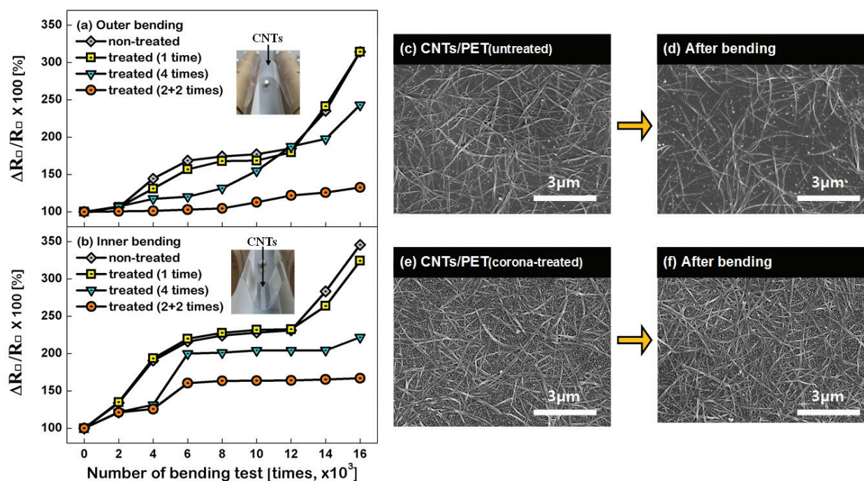
Figure 8. The changes in R_a of CNTs during bending: (a) for outer bending and (b) for inner bending. [(c)–(f)] The comparison of FE-SEM images for the CNTs before and after bending. The photos (c) and (d) indicate the CNTs deposited on the nontreated PET substrates. The photos (e) and (f) indicate the CNTs deposited on the [2+2]-times corona-treated PET substrates.
