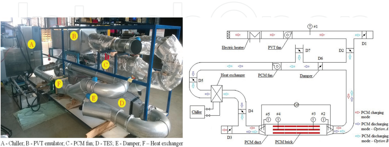
Figure 9. Laboratory-scale test rig of the PCM TES system.
