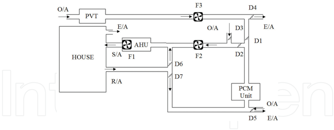
Figure 12. Schematic of the solar-assisted HVAC system (where S/A—supply air, O/A—outside air, R/A—return air, E/A—exhaust air, F—fan and D—damper) [32].
