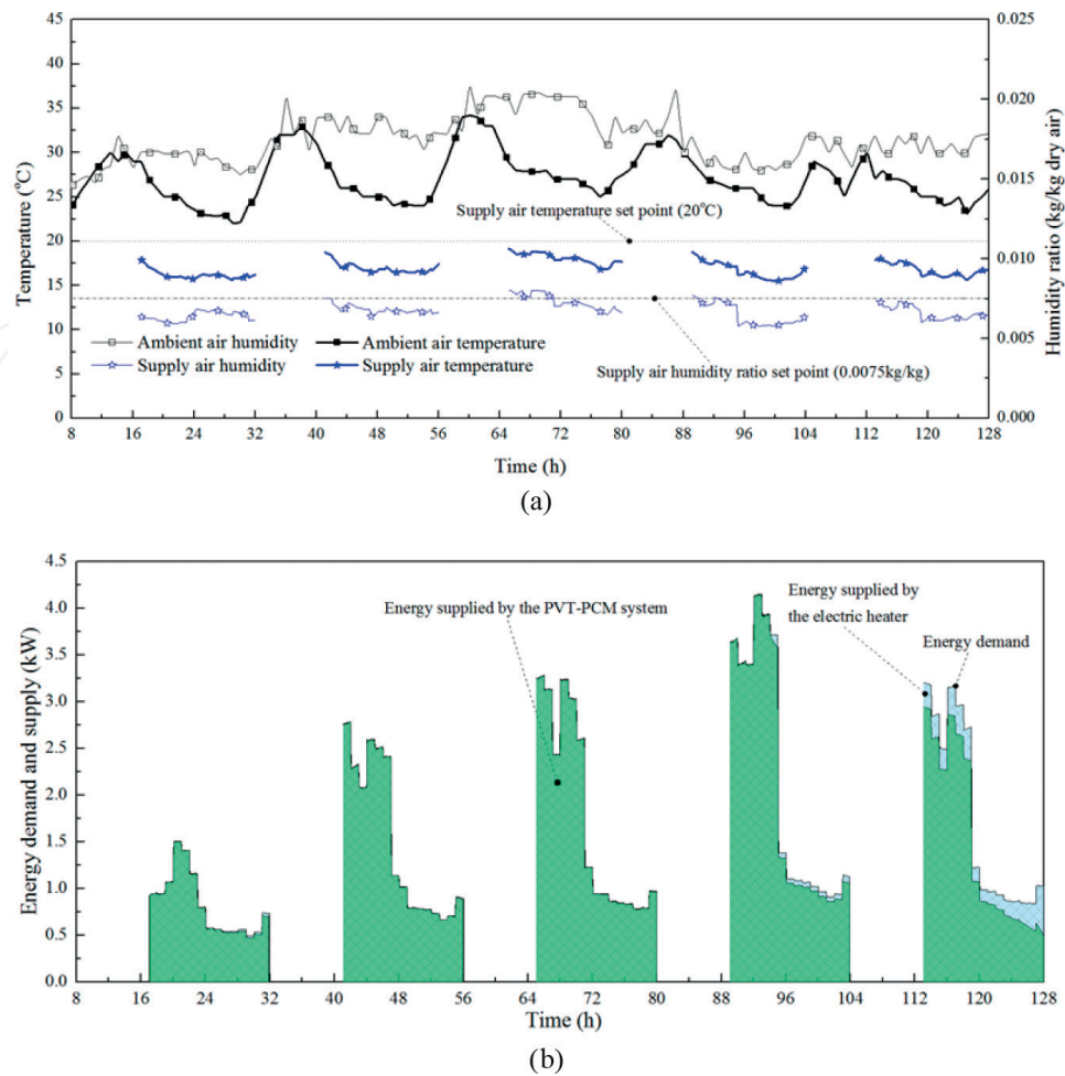
Figure 15. Simulation results of the rotary desiccant cooling system using PVT collectors and PCMs. (a) Ambient air and supply air conditions of the desiccant cooling system. (b) Energy required for desiccant wheel regeneration and energy supplied by the PVT-PCM system.
