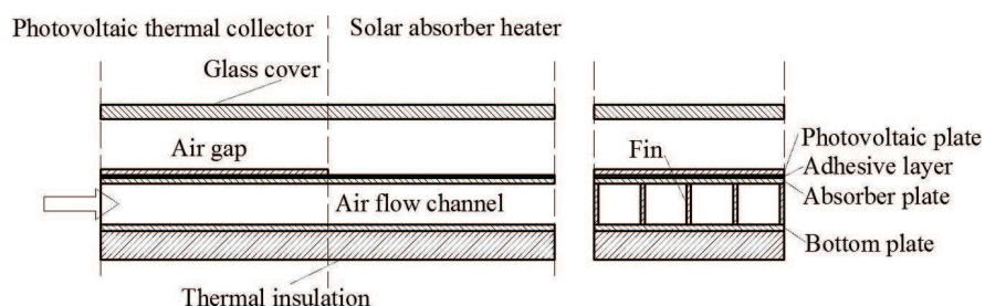
Figure 14. Schematic of the hybrid PVT-SAH system.
