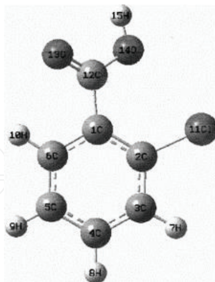
Figure 4. Numbering system implemented for 2-chlorobenzoic acid.
