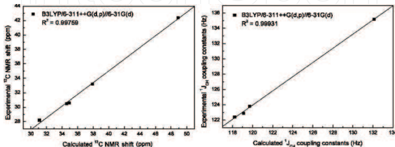
Figure 7. Plot of the calculated vs. the experimental ^{13}\text{C} NMR chemical shifts (ppm) and ^1J coupling constants (Hz) of danon.
