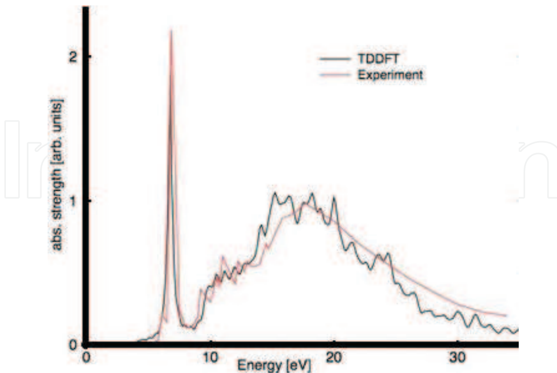
Figure 1. Absorption spectra of benzene.
