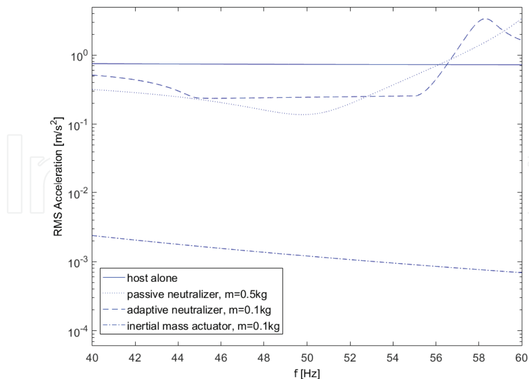
Figure 7. RMS acceleration of a vibrating host structure with different vibration control systems.
