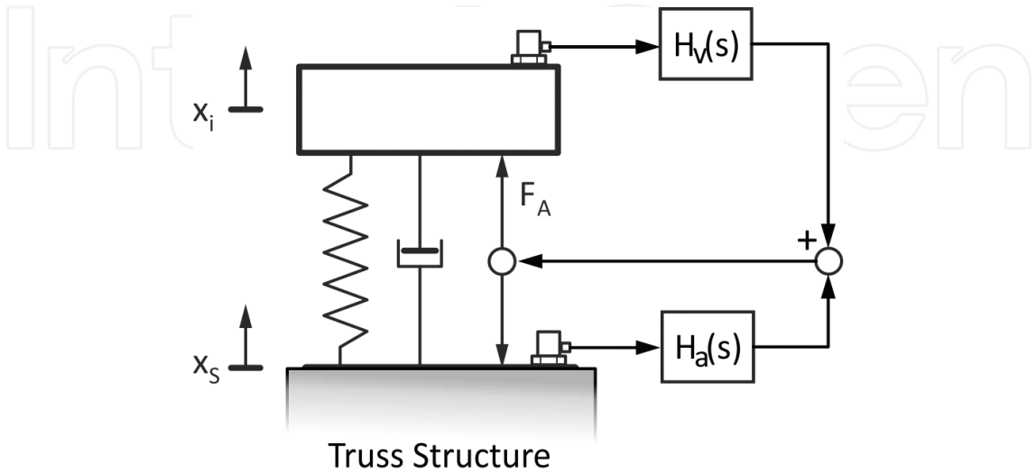
Figure 18. Block diagram of the control system.
