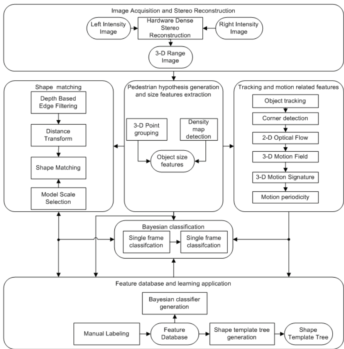
Fig. 19. Classification dataflow
