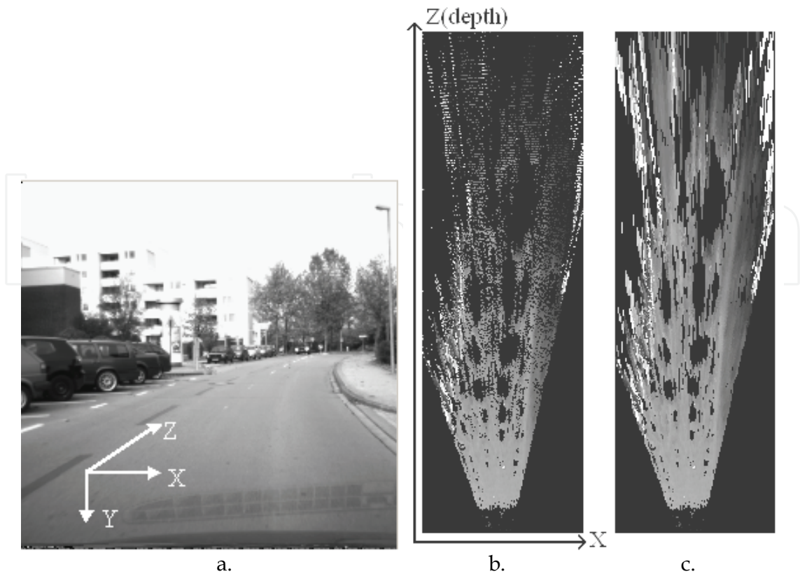
Fig. 15. The urban scenario (a) and the DEM (b. initial, c. with propagation of heights). Darker means more elevated.
