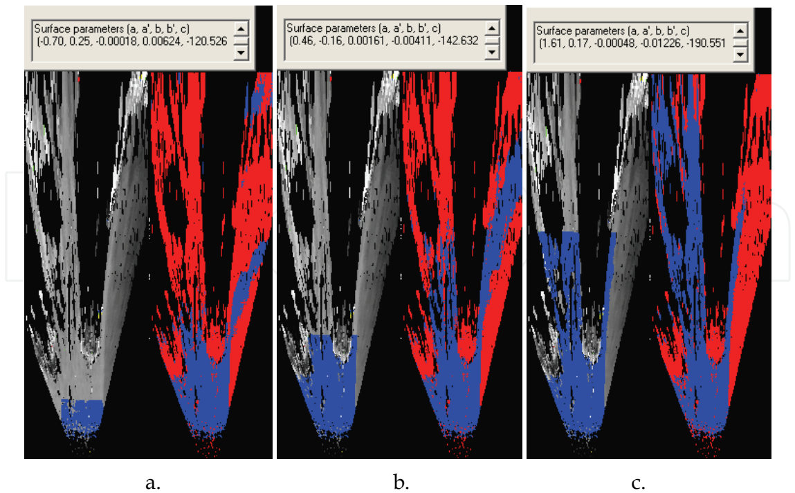
Fig. 17. Road inliers (blue) / outliers (red) detected with the primary surface in a. Intermediate regions, growing from left to right (b and c). For each image, the left side shows the inliers used for surface fitting, while the right side shows the classification of the whole DEM based on the current surface parameters.
