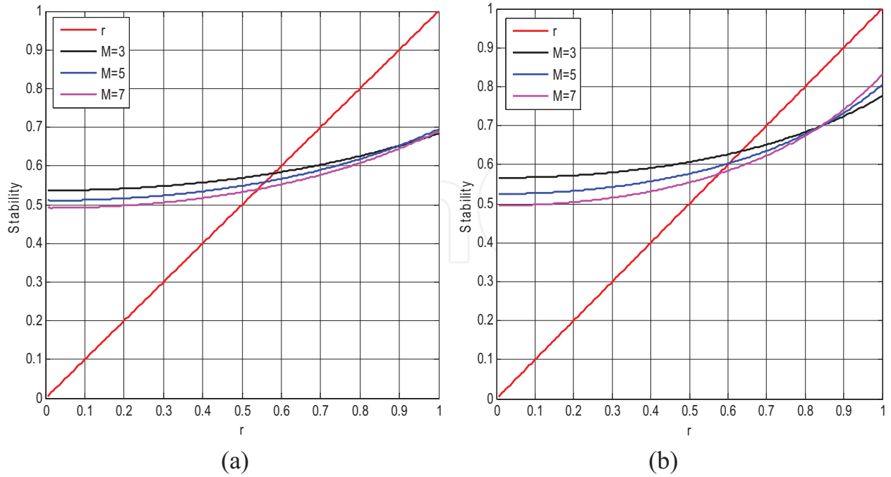
Figure 3. Stability condition in 2D. (a) The traditional staggered grid FD scheme and (b) the new staggered grid FD scheme.
