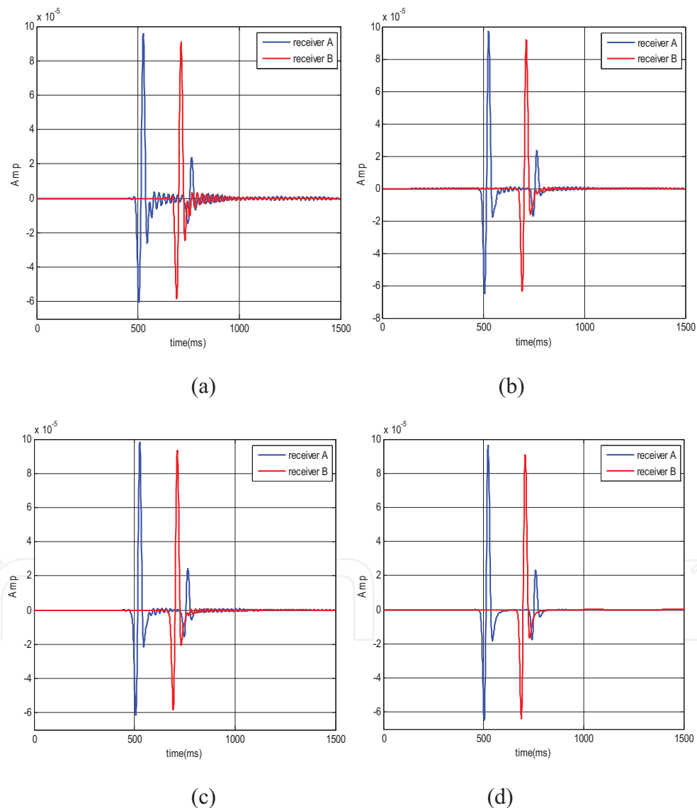
Figure 5. Seismograms recorded by different simulation methods. (a) The traditional staggered grid FD scheme with FD coefficients determined in the space domain by Taylor expansion method, (b) the traditional staggered grid FD scheme with FD coefficients determined in the space domain by least squares method, (c) the new staggered grid FD scheme with FD coefficients determined in the time-space domain by the linear method, and (d) the pseudo-spectrum method.
