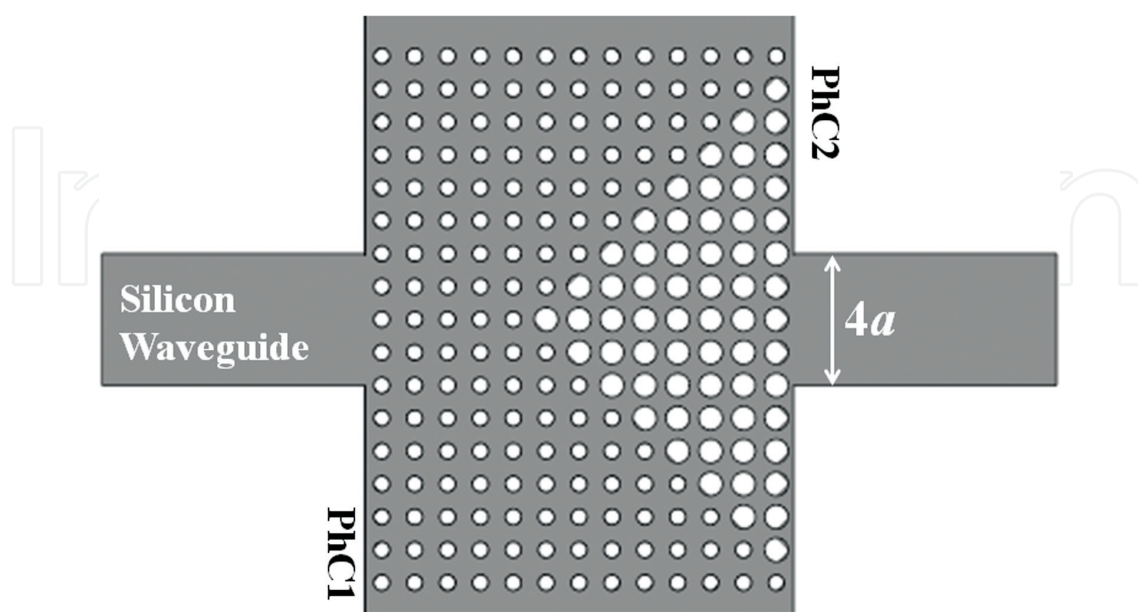
Figure 13. Optical diode with PhC heterostructure connecting standard silicon waveguide [29].
