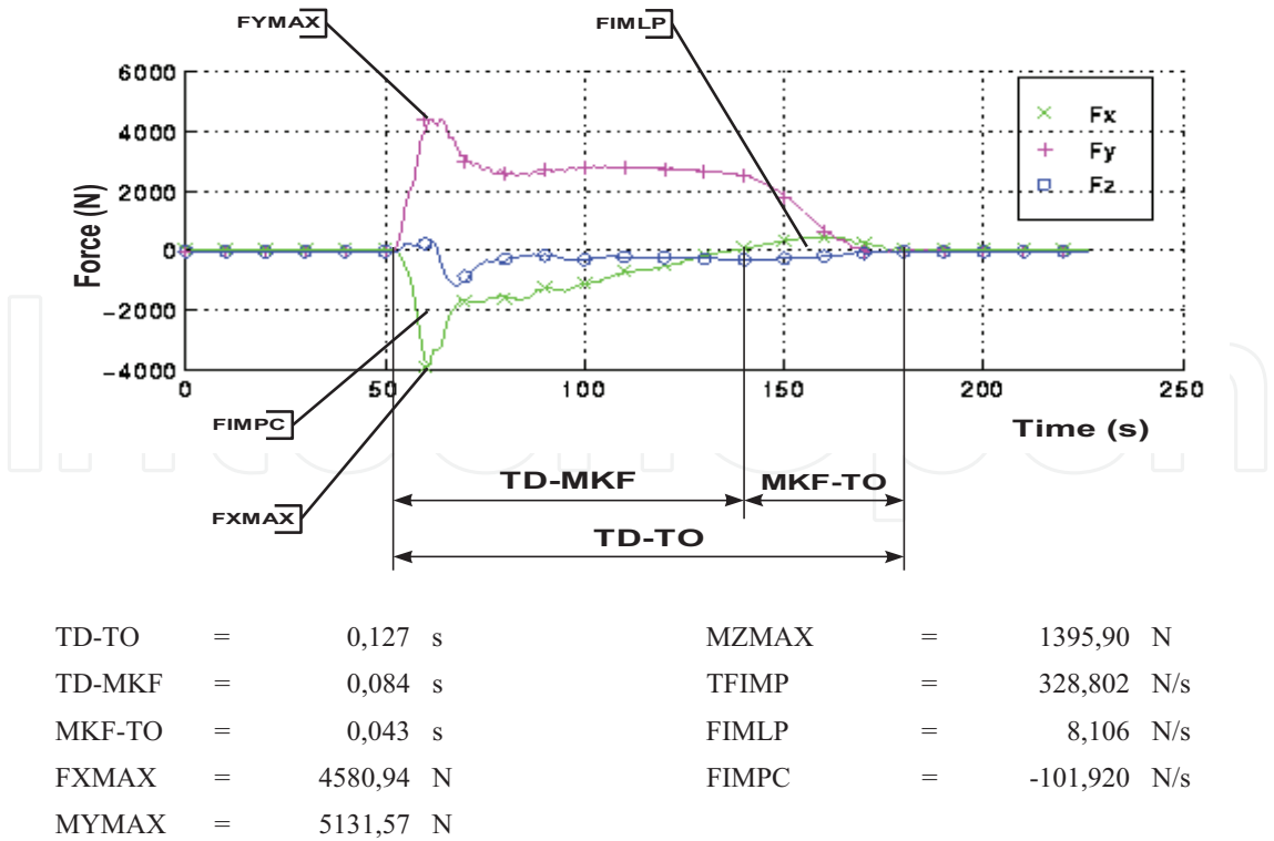
Figure 7. Force diagram of the take-off phase.
