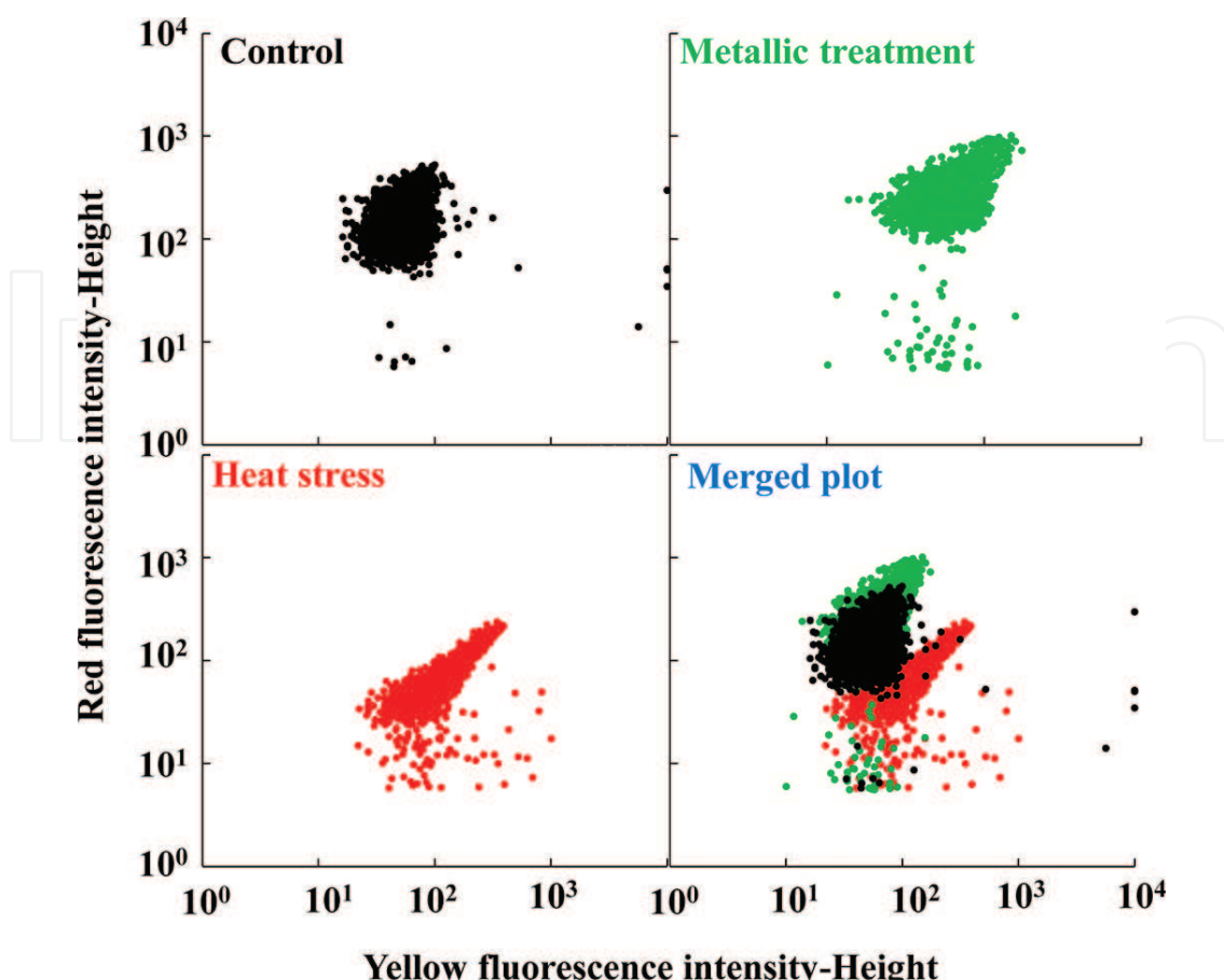
Figure 7. Distribution of Chlorella obtained using FCM on a graph of the red fluorescence intensity vs. the yellow fluorescence intensity, modified from the literature [1, 12–14]. The heat stress and the metallic treatment samples, respectively, derive from algae treated with heat and algae treated with a metallic solution containing concentrations of eluate of 50 vol%.
