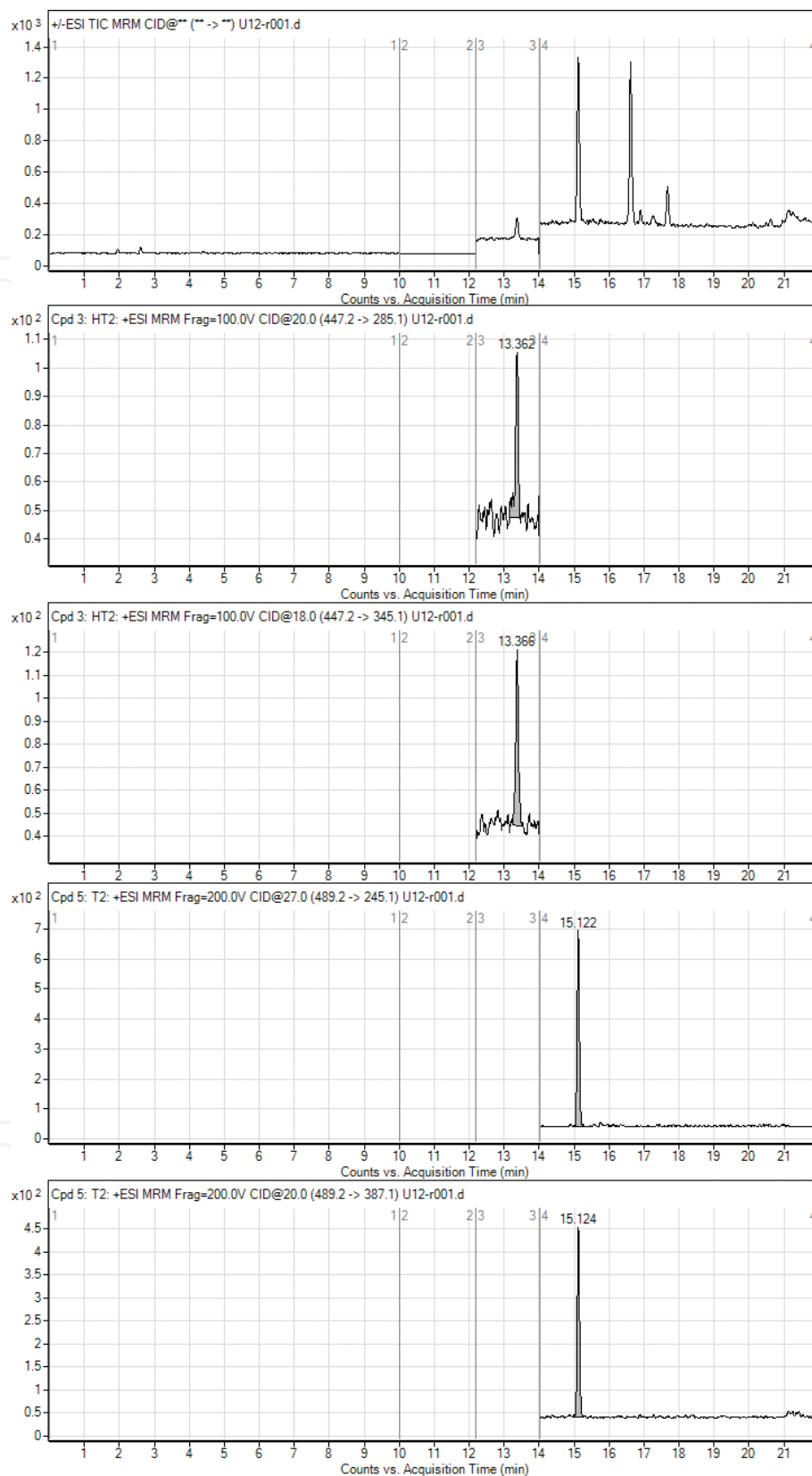
Figure 1. A typical LC-MS/MS-MRM chromatogram of the certified reference material (CRM, oat flour) with values of 77.9 \mu\text{g/kg} determined for T-2 and 75.6 \mu\text{g/kg} determined for HT-2; TIC; HT-2 MRM 447.2 \rightarrow 285.1; HT-2 MRM 447.2 \rightarrow 345.1; T-2 MRM 489.2 \rightarrow 245.1; and T-2 MRM 489.2 \rightarrow 387.1.
