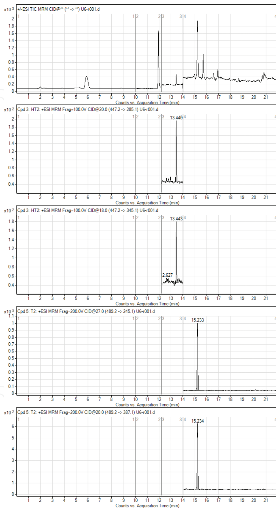
Figure 2. A typical LC-MS/MS-MRM chromatogram of the contaminated maize sample subsequently subjected to thermal reduction processing (128 µg/kg of T-2 and 256 µg/kg of HT-2); TIC; HT-2 MRM 447.2 → 285.1; HT-2 MRM 447.2 → 345.1; T-2 MRM 489.2 → 245.1; and T-2 MRM 489.2 → 387.1.
