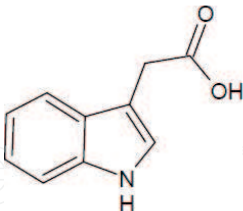
Figure 3. Indole-3-acetic acid (AIA) which is the main naturally occurring auxin. Source: Raven [14].
