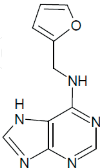
Figure 4. Molecule of kinetin that probably does not occur naturally in plants. Source: Raven [14].
