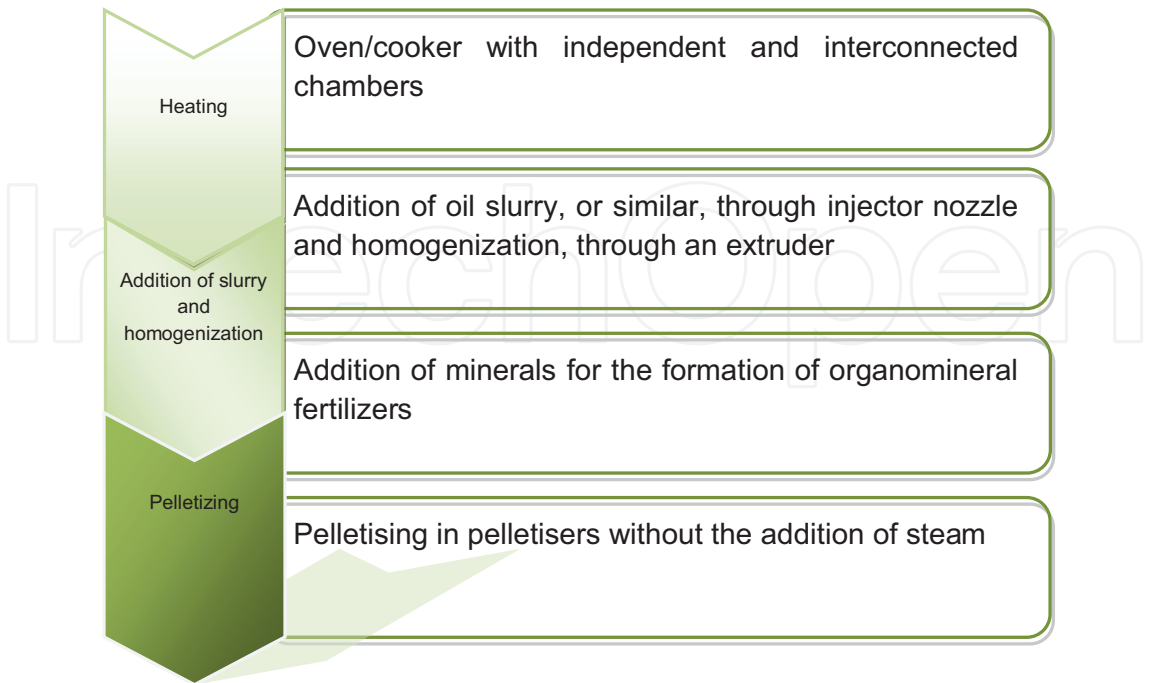
Figure 2. Flowchart of the physical-chemical-mechanical process of digestion and avian bed pelletization for the production of organic compound and organo-mineral fertilizers. Source: de Oliveira [8].
