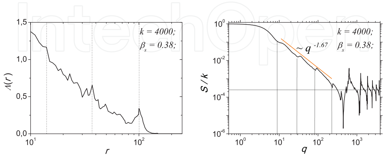
Figure 12. Left part: the lacunarity of pentaflake fractal; right part: the structure factor of pentaflake fractal.
