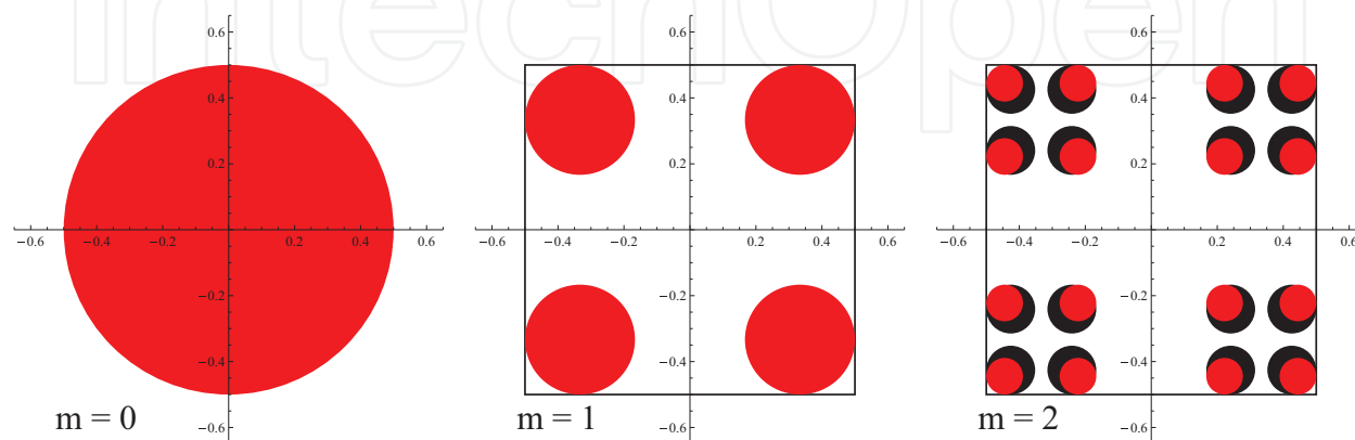
Figure 7. Construction of the Cantor-like fat fractal.
