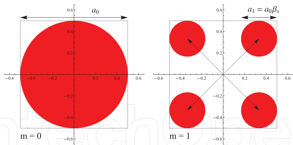
Figure 4. The rule of the deterministic mass-fractal construction.
