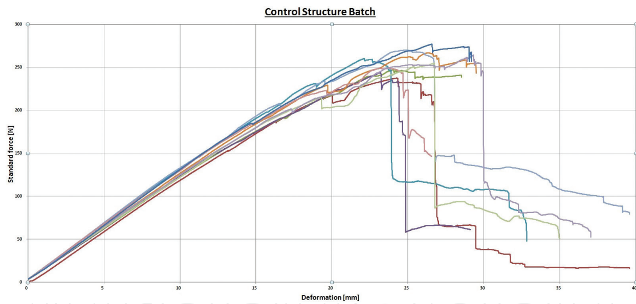
Figure 3. Collective data of three point flexural test.
