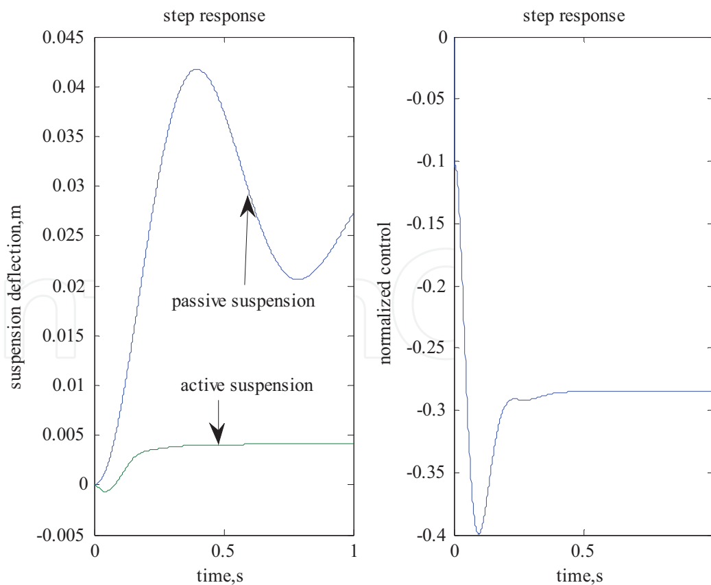
Figure 6. Step response at light load.
