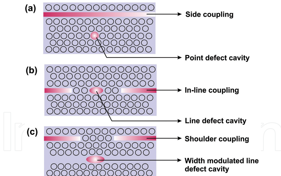
Figure 4. Schematic representation of nanocavities along with various coupling schemes: (a) a point-defect nanocavity with side coupling with the waveguide, (b) a line-defect nanocavity with in-line coupling with the waveguide, and (c) a width-modulated line defect nanocavity with shoulder coupling with the waveguide.
