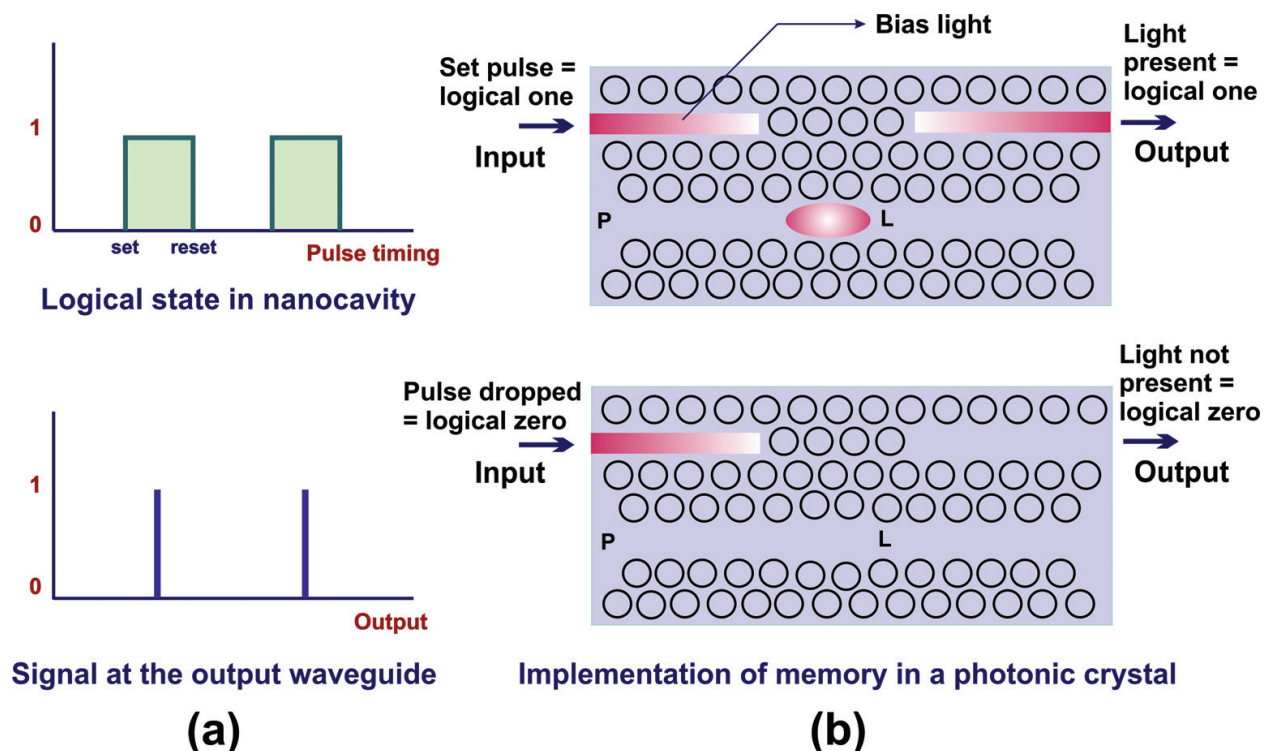
Figure 9. (a) Logical state of nanocavity and its indication in the output waveguide, and (b) implementation of memory in photonic crystal.
