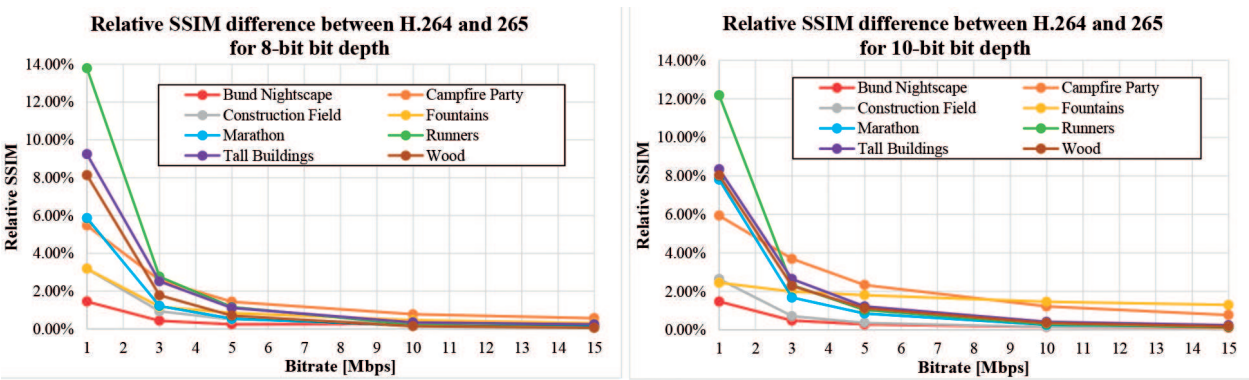
Figure 13. Relative SSIM difference between H.264 and H.265 compression standards for 8-bit (left) and 10-bit bit depth (right) in FHD.
