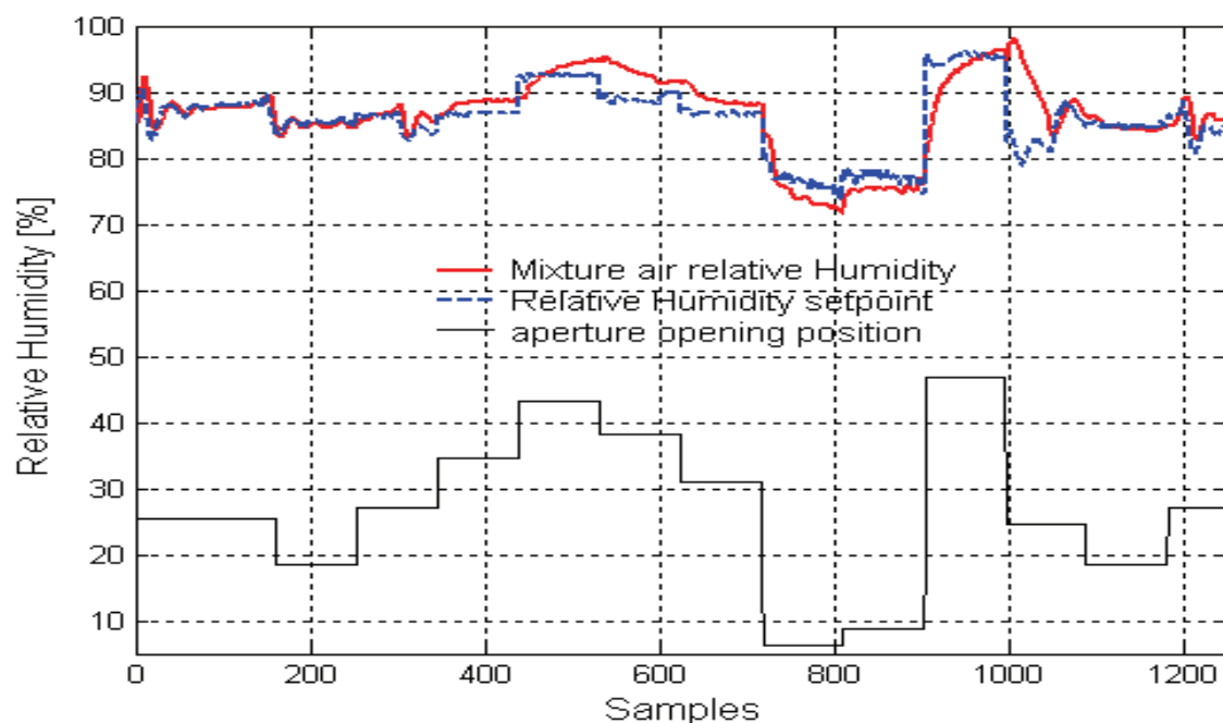
Fig. 12. Relative humidity of the mixture air
