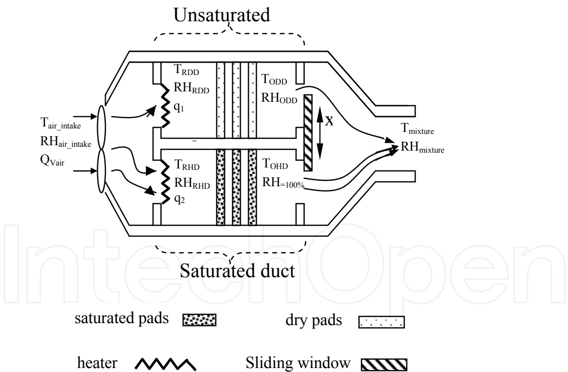
Fig. 2. Air-conditioning system
