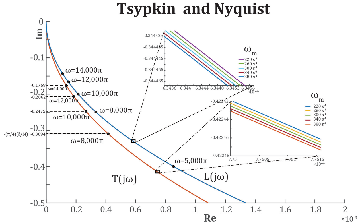
Figure 6. Graphical solution using Tsyppkin's method.
