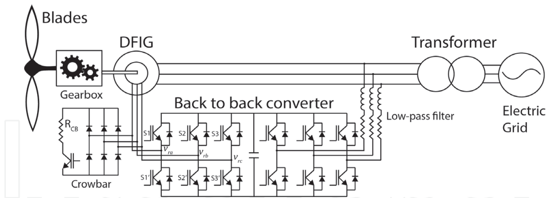
Figure 2. Basic scheme of DFIG-based wind turbine.
