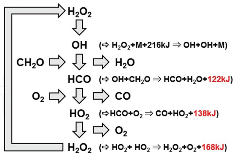
Figure 5. Schematic of H 2 O 2 reaction loop [24].
