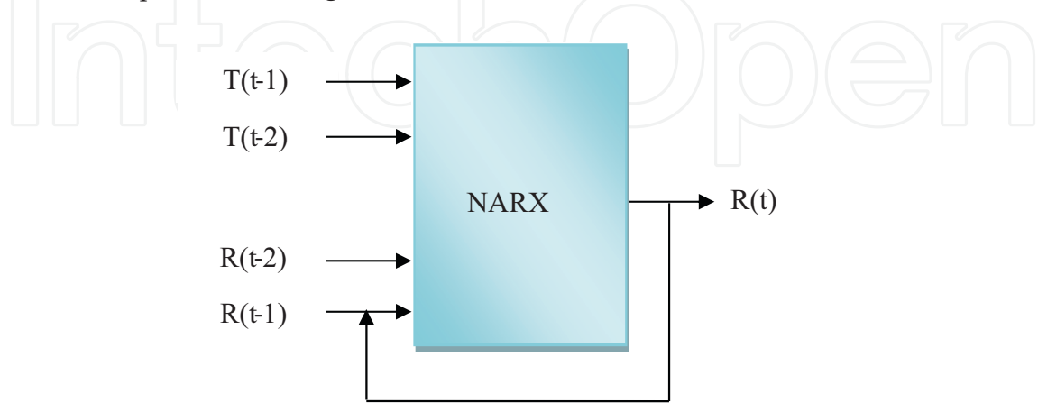
Figure 12. Neural architecture for the NARX model.
