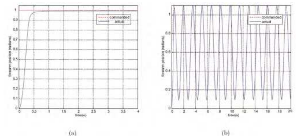
Fig. 11. Position control of the forearm position controller: (a) Step response to a reference signal with a step of 1 rad shows no overshoot and quick, non-oscillatory response. (b) Trajectory following behavior when tracking a 4 rad/s sinusoidal reference signal of amplitude 0.5 rad centered at 0.6 rad demonstrates that the device bandwidth matches human capabilities.
