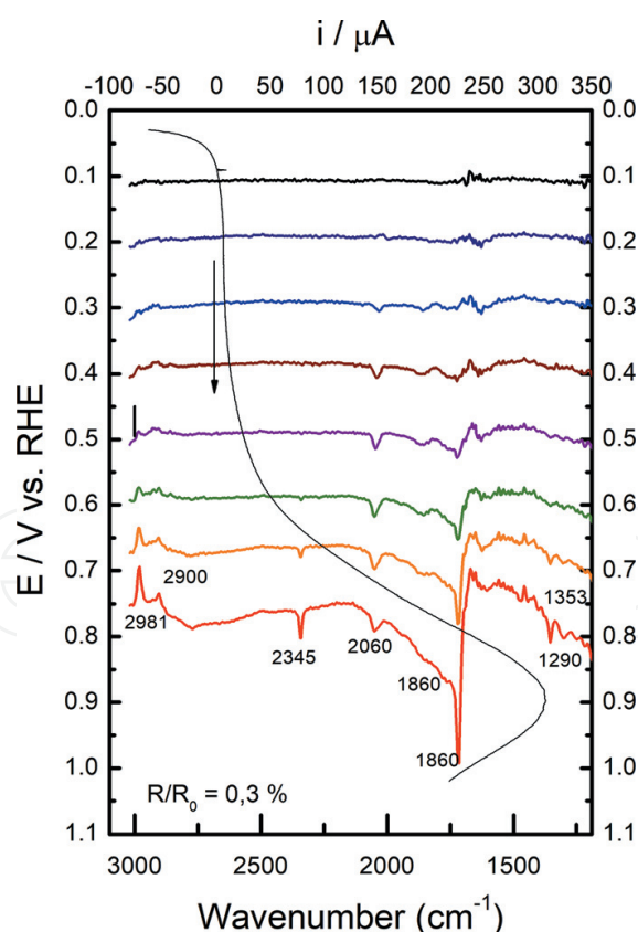
Figure 9. Linear sweep voltammetry and FTIR registered on Pt catalysts in 0.5 mol L -1 H 2 SO 4 and 0.5 mol L -1 CH 3 CH 2 OH, at room temperature, v(\text{lsv}) = 1 \text{ mV}^{-1} and FTIR measurements carried out in a mixture of 0.1 HClO 4 (mol L -1 ) and CH 3 CH 2 OH (0.1 mol L -1 ).
