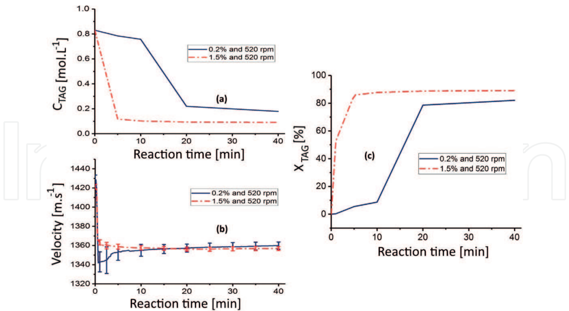
Figure 10. Variation of (a) TAG concentration, (b) propagation velocity and (c) TAG conversion for the reactions with 520 rpm of rotation.
