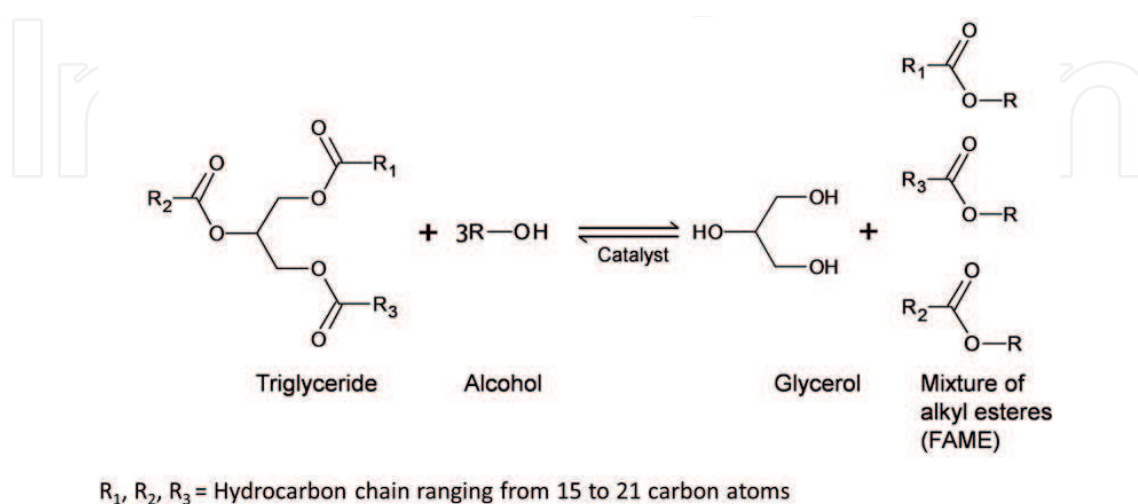
Figure 1. Transesterification of vegetable oil for biodiesel production.
