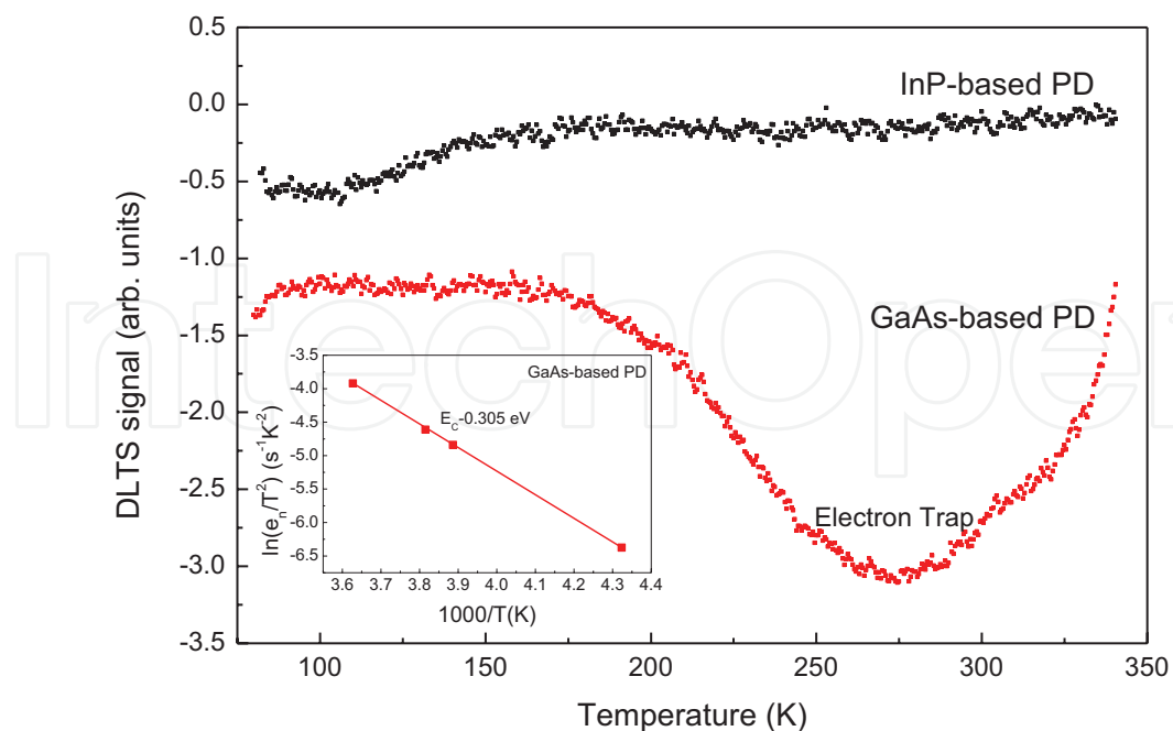
Figure 20. DLTS spectra for the two samples measured at a rate window of 680 Hz. Inset: Arrhenius plot of the deep state observed in GaAs-based PD sample using different lock-in frequencies of 41 Hz, 240 Hz, 320 Hz and 680 Hz. Reprinted with permission from Elsevier.
