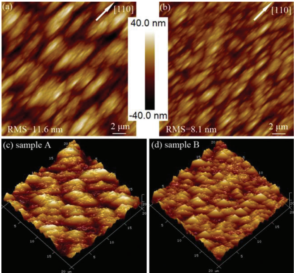
Figure 22. AFM images of samples A and B. The scan area is 20 × 20 \mu\text{m}^2 . Reprinted with permission from Elsevier.
