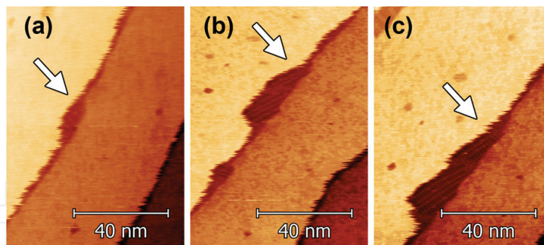
Figure 11. Evolution over 5 min of the sample at 1000 K, showing the growth of a carbon reconstruction patch, displacing the Tm layer: (a) At the beginning, (b) the time between and (c) at the end of the sequence.
