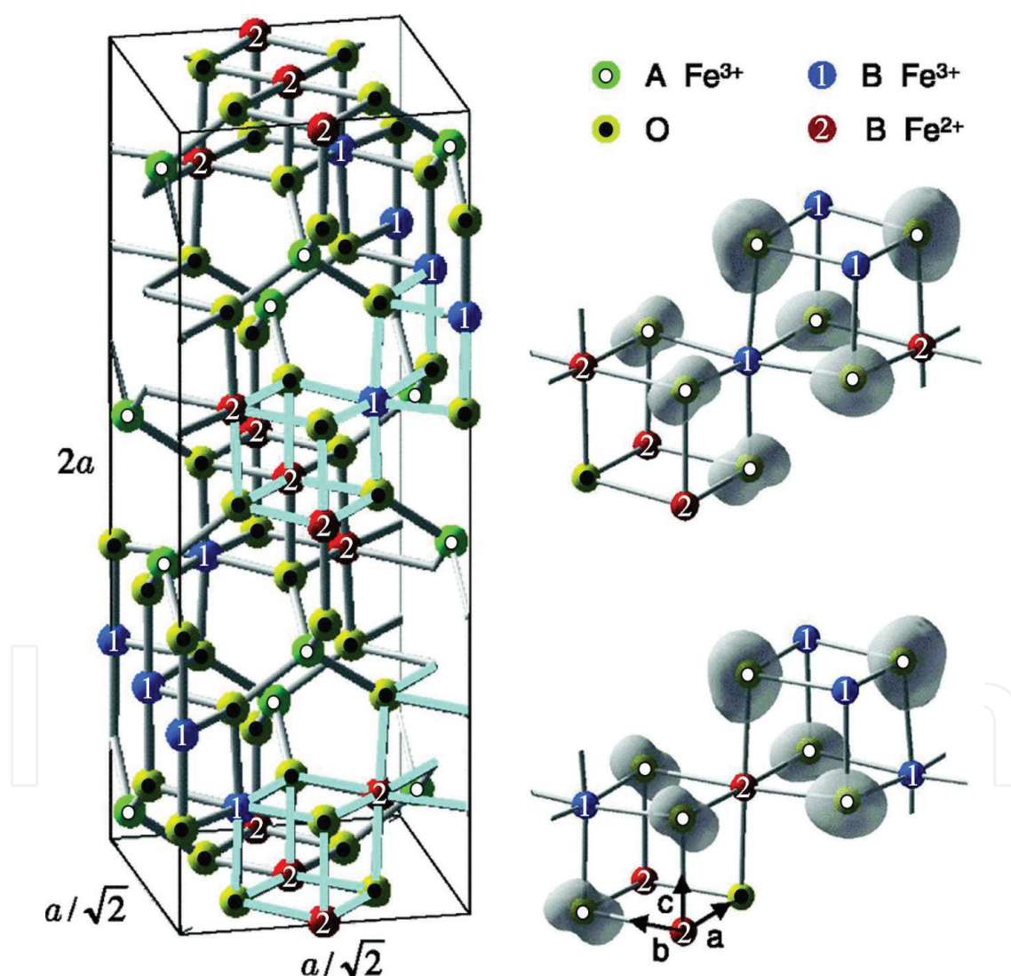
Figure 5. Left: monoclinic crystal structure of \text{Fe}_3\text{O}_4 in the low-temperature phase corresponding to a subcell of a_2 \times a_2 \times 2a with P2/c symmetry. Right: 3D isosurfaces of unoccupied density of states of the O 2p integrated between the fermi level and 1 eV above within the corresponding \text{Fe}_3\text{O}_4 cubes highlighted in the crystal structure. For simplicity, we denote the octahedral Fe site with nominal 2+ and 3+ valences as \text{Fe}^{2+} and \text{Fe}^{3+} , respectively [22].
