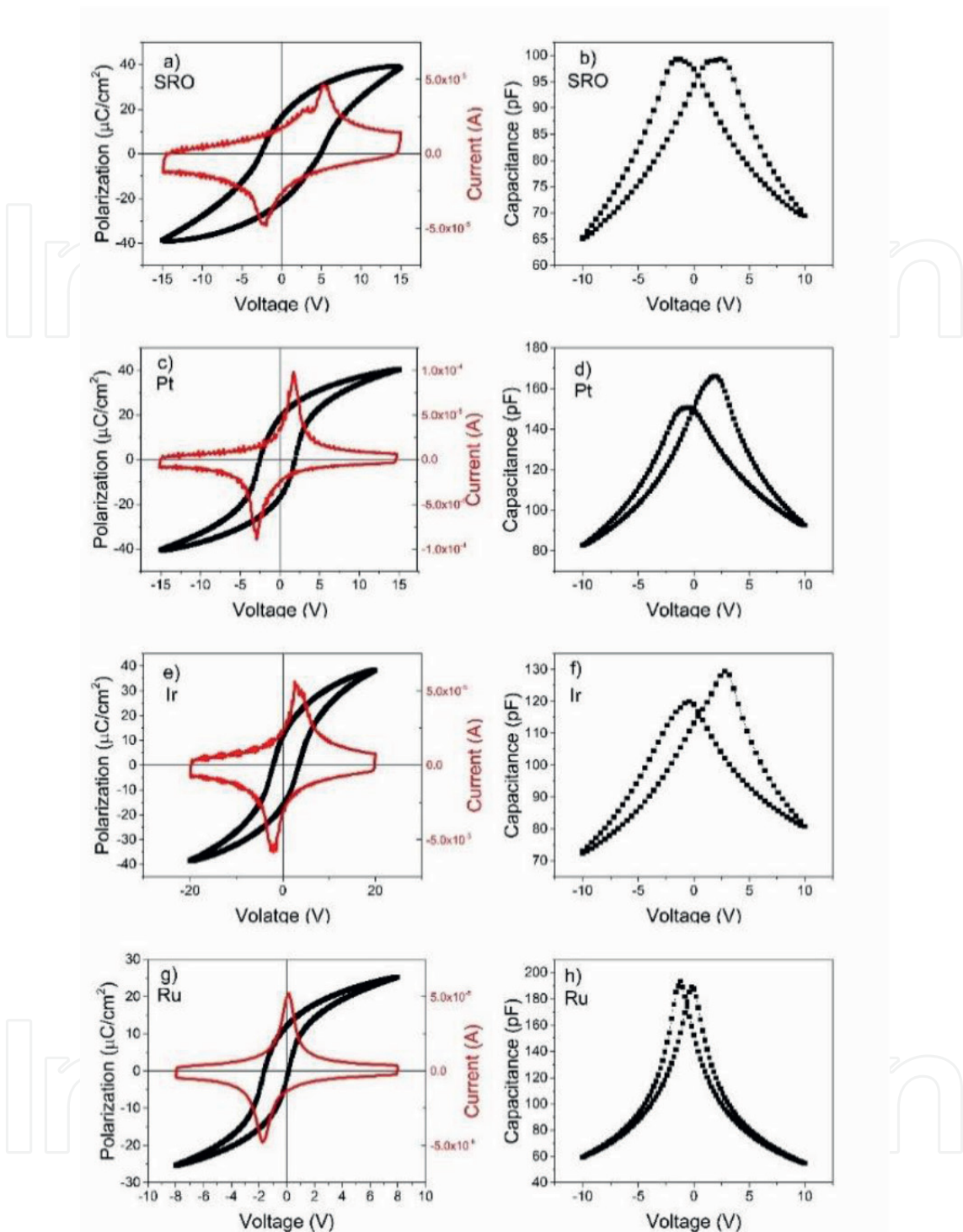
Figure 8. Hysteresis loops and capacitance-voltage characteristics obtained for different top electrodes: (a,b) for SRO, (c,d) for Pt, (e,f) for Ir and (g,h) for Ru, respectively.
